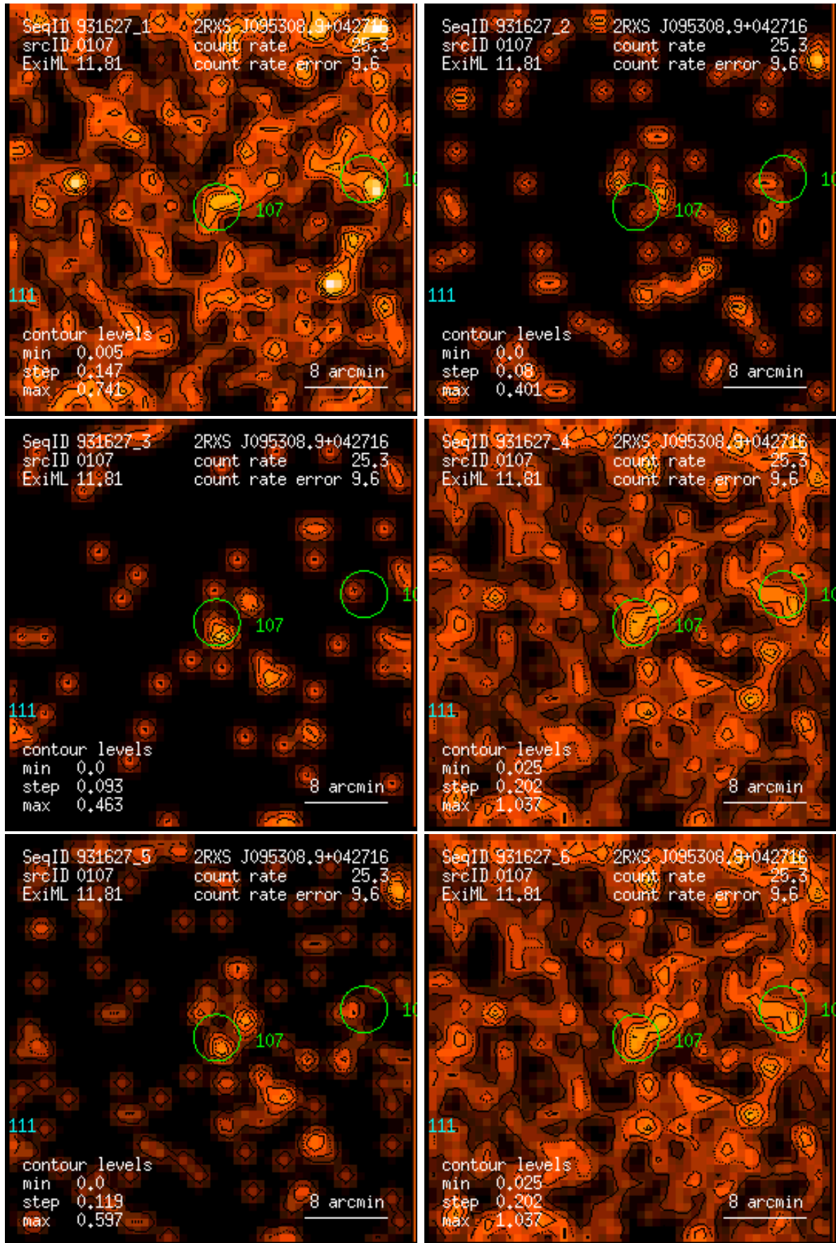
Figure 107: RASS 931627: detection 0107: band rate images, Gaussian filter: (1) PSPC channels 11 – 41, (2) 52 – 90, (3) 91 – 201, (4) 11 – 235, (5) 52 – 201, (6) 11 – 201. Broad band rates in counts/ks. Band rate contour levels in counts/ks/arcmin 2 .
