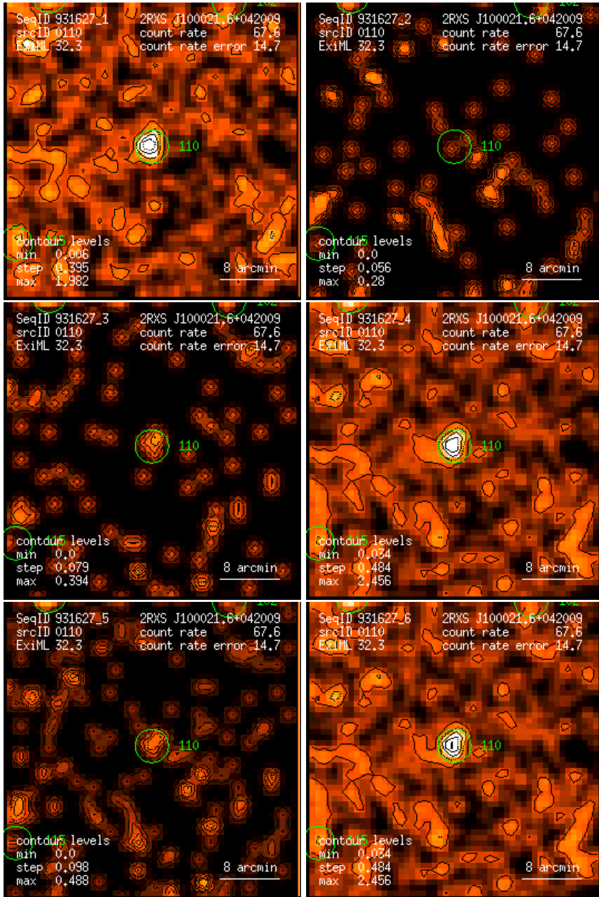
Figure 110: RASS 931627: detection 0110: band rate images, Gaussian filter: (1) PSPC channels 11 – 41, (2) 52 – 90, (3) 91 – 201, (4) 11 – 235, (5) 52 – 201, (6) 11 – 201. Broad band rates in counts/ks. Band rate contour levels in counts/ks/arcmin 2 .
