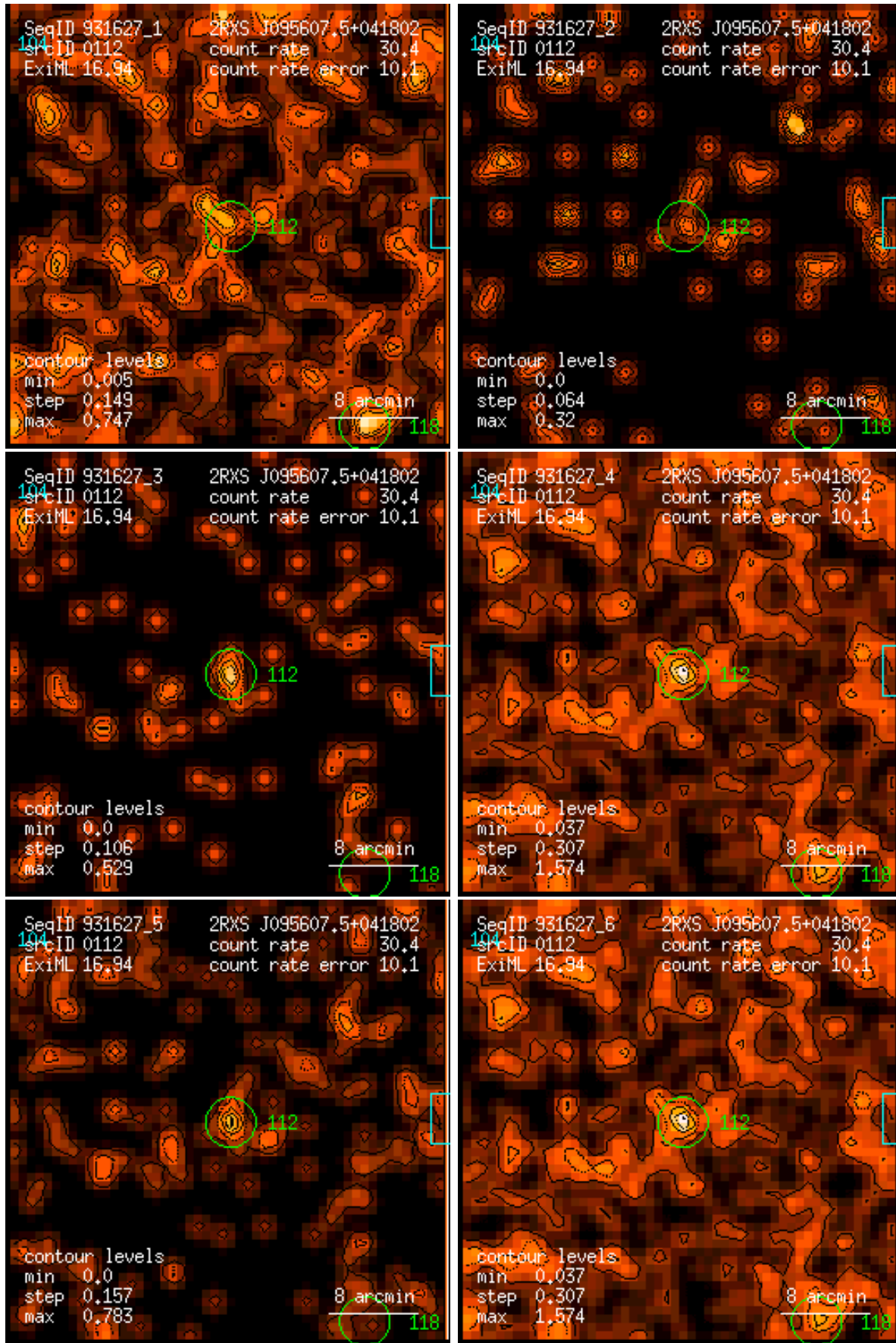
Figure 112: RASS 931627: detection 0112: band rate images, Gaussian filter: (1) PSPC channels 11 – 41, (2) 52 – 90, (3) 91 – 201, (4) 11 – 235, (5) 52 – 201, (6) 11 – 201. Broad band rates in counts/ks. Band rate contour levels in counts/ks/arcmin 2 .
