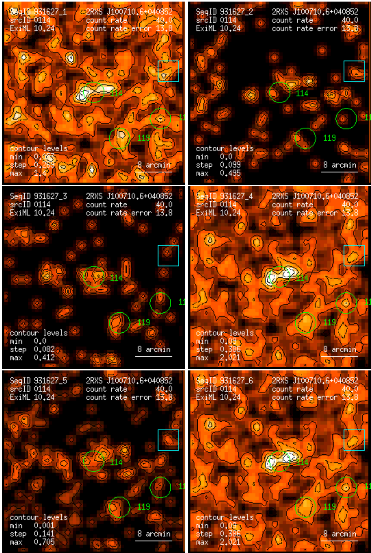
Figure 114: RASS 931627: detection 0114: band rate images, Gaussian filter: (1) PSPC channels 11 – 41, (2) 52 – 90, (3) 91 – 201, (4) 11 – 235, (5) 52 – 201, (6) 11 – 201. Broad band rates in counts/ks. Band rate contour levels in counts/ks/arcmin 2 .
