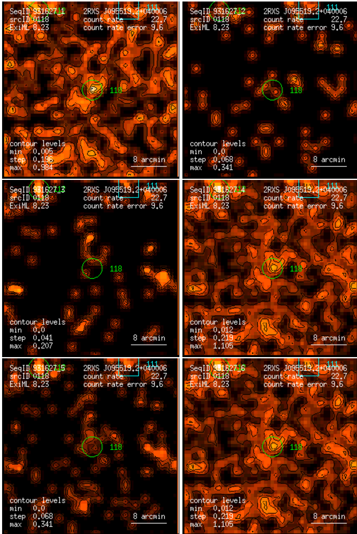
Figure 118: RASS 931627: detection 0118: band rate images, Gaussian filter: (1) PSPC channels 11 – 41, (2) 52 – 90, (3) 91 – 201, (4) 11 – 235, (5) 52 – 201, (6) 11 – 201. Broad band rates in counts/ks. Band rate contour levels in counts/ks/arcmin 2 .
