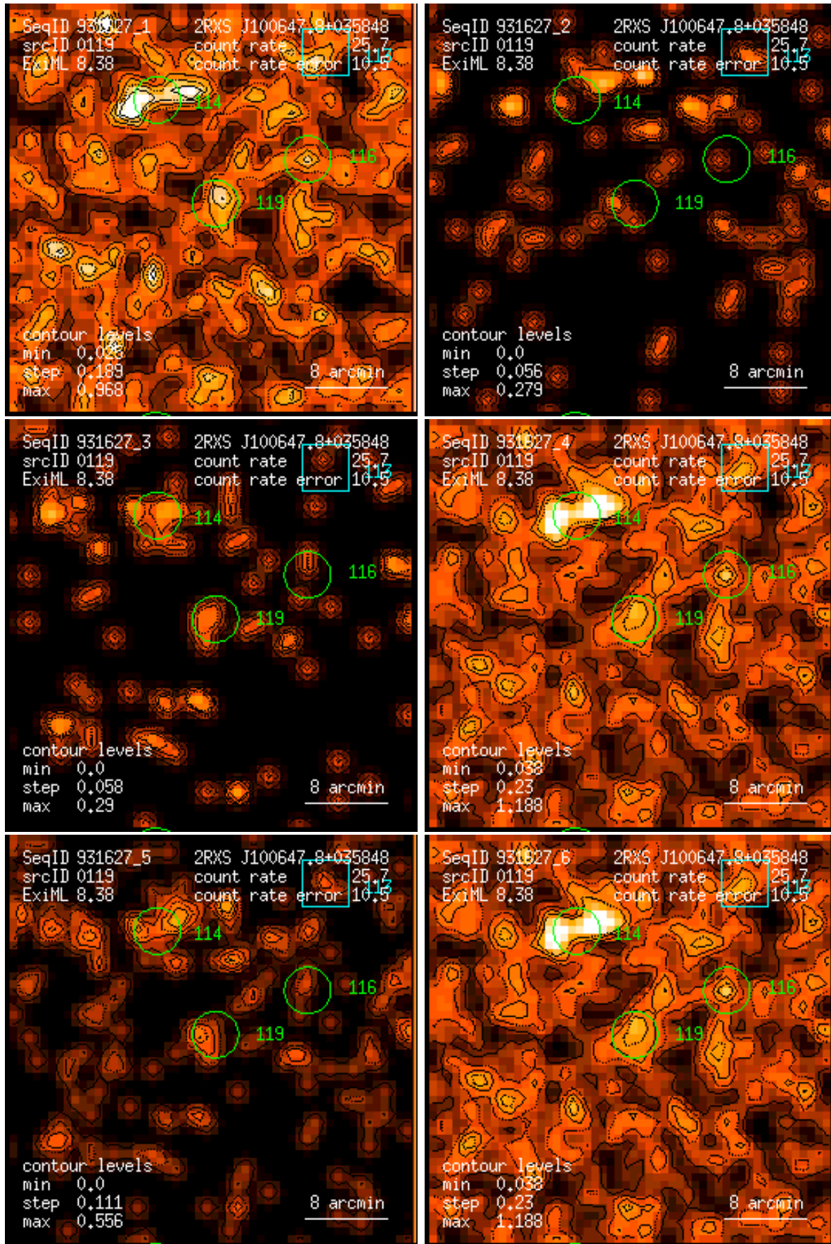
Figure 119: RASS 931627: detection 0119: band rate images, Gaussian filter: (1) PSPC channels 11 – 41, (2) 52 – 90, (3) 91 – 201, (4) 11 – 235, (5) 52 – 201, (6) 11 – 201. Broad band rates in counts/ks. Band rate contour levels in counts/ks/arcmin 2 .
