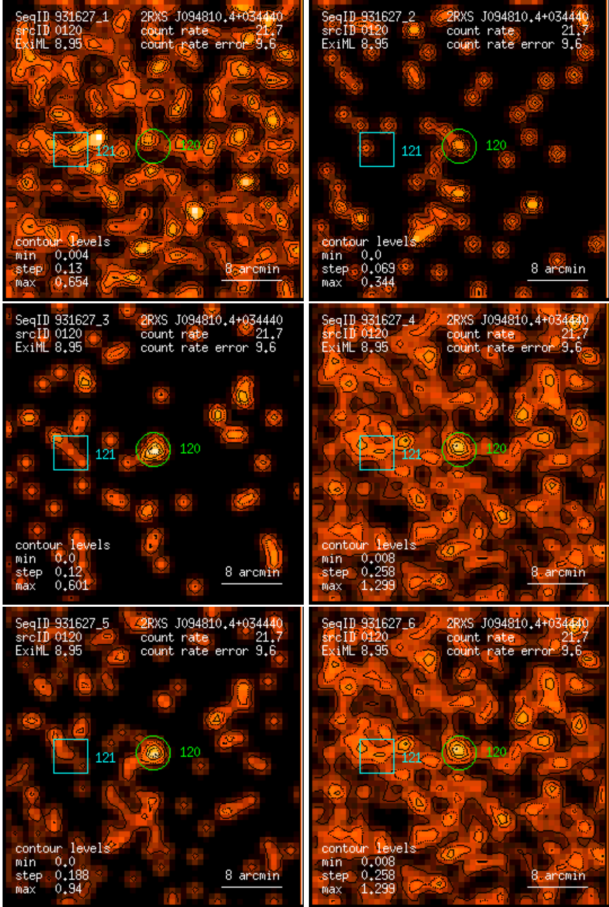
Figure 120: RASS 931627: detection 0120: band rate images, Gaussian filter: (1) PSPC channels 11 – 41, (2) 52 – 90, (3) 91 – 201, (4) 11 – 235, (5) 52 – 201, (6) 11 – 201. Broad band rates in counts/ks. Band rate contour levels in counts/ks/arcmin 2 .
