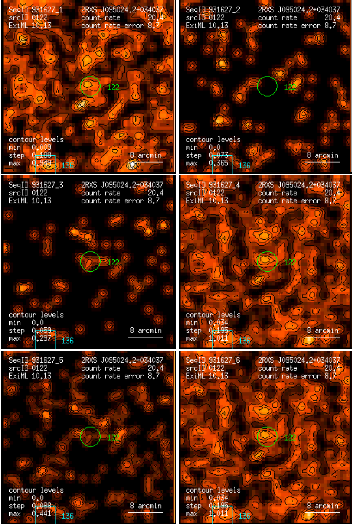
Figure 122: RASS 931627: detection 0122: band rate images, Gaussian filter: (1) PSPC channels 11 – 41, (2) 52 – 90, (3) 91 – 201, (4) 11 – 235, (5) 52 – 201, (6) 11 – 201. Broad band rates in counts/ks. Band rate contour levels in counts/ks/arcmin 2 .
