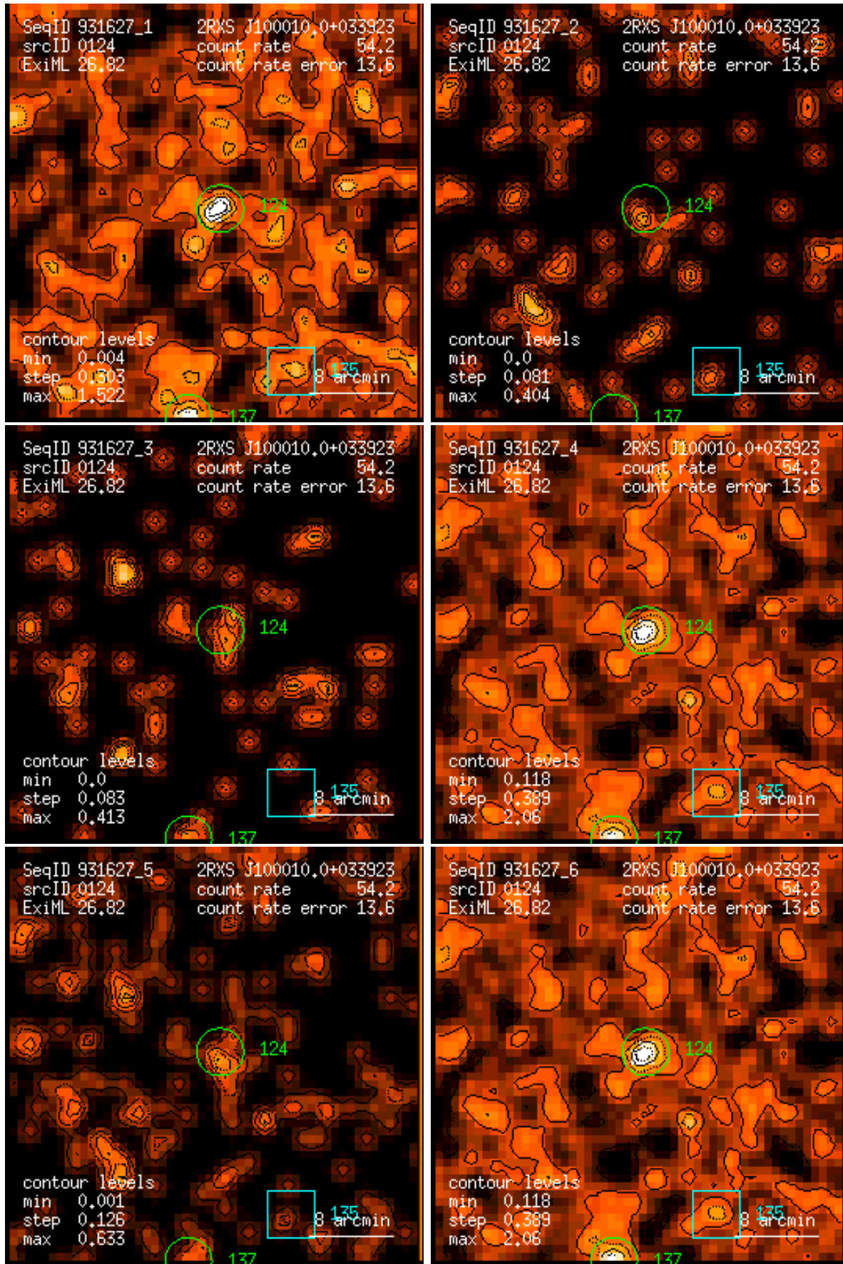
Figure 124: RASS 931627: detection 0124: band rate images, Gaussian filter: (1) PSPC channels 11 – 41, (2) 52 – 90, (3) 91 – 201, (4) 11 – 235, (5) 52 – 201, (6) 11 – 201. Broad band rates in counts/ks. Band rate contour levels in counts/ks/arcmin 2 .
