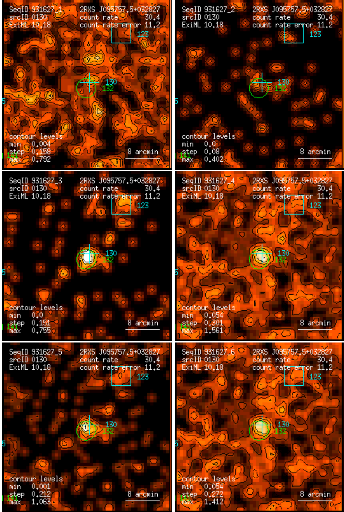
Figure 130: RASS 931627: detection 0130: band rate images, Gaussian filter: (1) PSPC channels 11 – 41, (2) 52 – 90, (3) 91 – 201, (4) 11 – 235, (5) 52 – 201, (6) 11 – 201. Broad band rates in counts/ks. Band rate contour levels in counts/ks/arcmin 2 .
