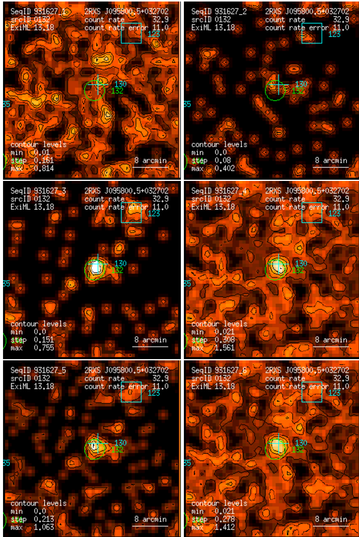
Figure 132: RASS 931627: detection 0132: band rate images, Gaussian filter: (1) PSPC channels 11 – 41, (2) 52 – 90, (3) 91 – 201, (4) 11 – 235, (5) 52 – 201, (6) 11 – 201. Broad band rates in counts/ks. Band rate contour levels in counts/ks/arcmin 2 .
