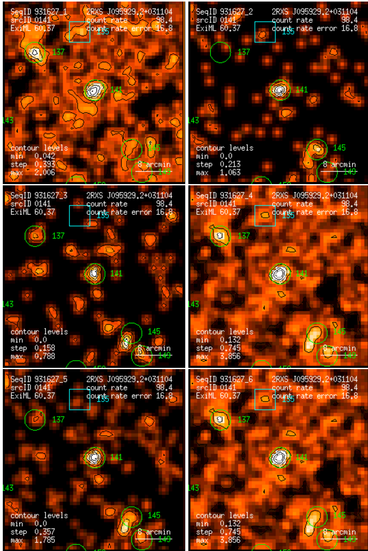
Figure 141: RASS 931627: detection 0141: band rate images, Gaussian filter: (1) PSPC channels 11 – 41, (2) 52 – 90, (3) 91 – 201, (4) 11 – 235, (5) 52 – 201, (6) 11 – 201. Broad band rates in counts/ks. Band rate contour levels in counts/ks/arcmin 2 .
