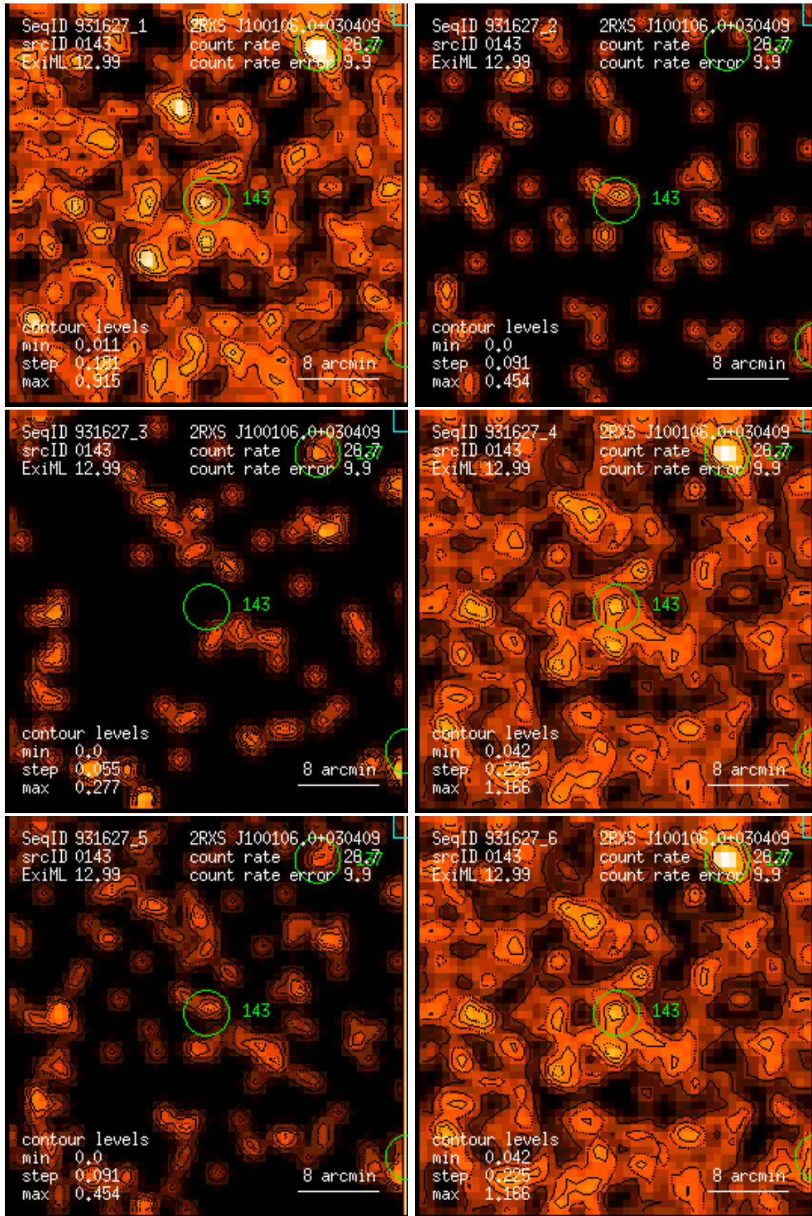
Figure 143: RASS 931627: detection 0143: band rate images, Gaussian filter: (1) PSPC channels 11 – 41, (2) 52 – 90, (3) 91 – 201, (4) 11 – 235, (5) 52 – 201, (6) 11 – 201. Broad band rates in counts/ks. Band rate contour levels in counts/ks/arcmin 2 .
