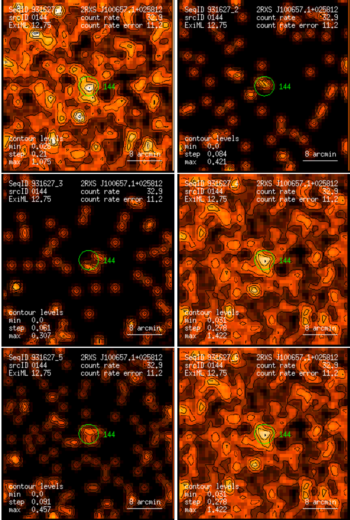
Figure 144: RASS 931627: detection 0144: band rate images, Gaussian filter: (1) PSPC channels 11 – 41, (2) 52 – 90, (3) 91 – 201, (4) 11 – 235, (5) 52 – 201, (6) 11 – 201. Broad band rates in counts/ks. Band rate contour levels in counts/ks/arcmin 2 .
