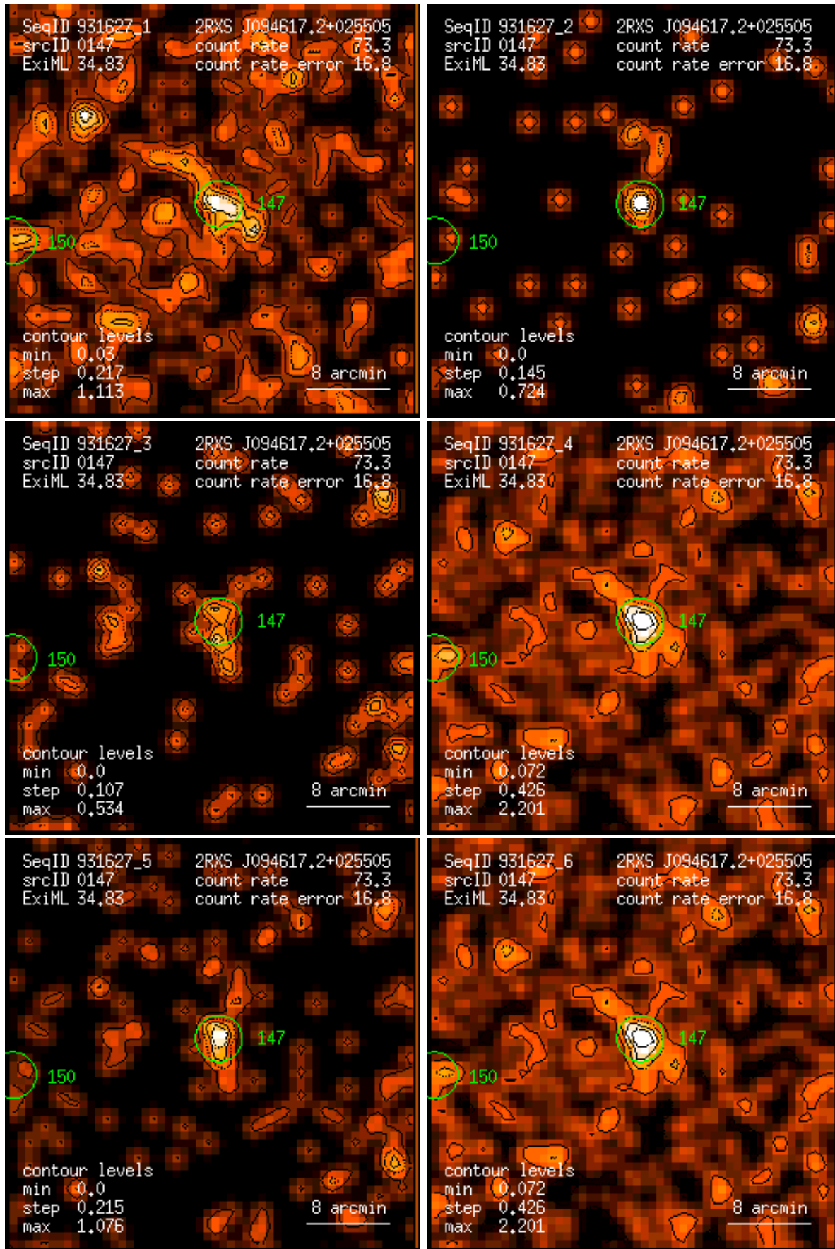
Figure 147: RASS 931627: detection 0147: band rate images, Gaussian filter: (1) PSPC channels 11 – 41, (2) 52 – 90, (3) 91 – 201, (4) 11 – 235, (5) 52 – 201, (6) 11 – 201. Broad band rates in counts/ks. Band rate contour levels in counts/ks/arcmin 2 .
