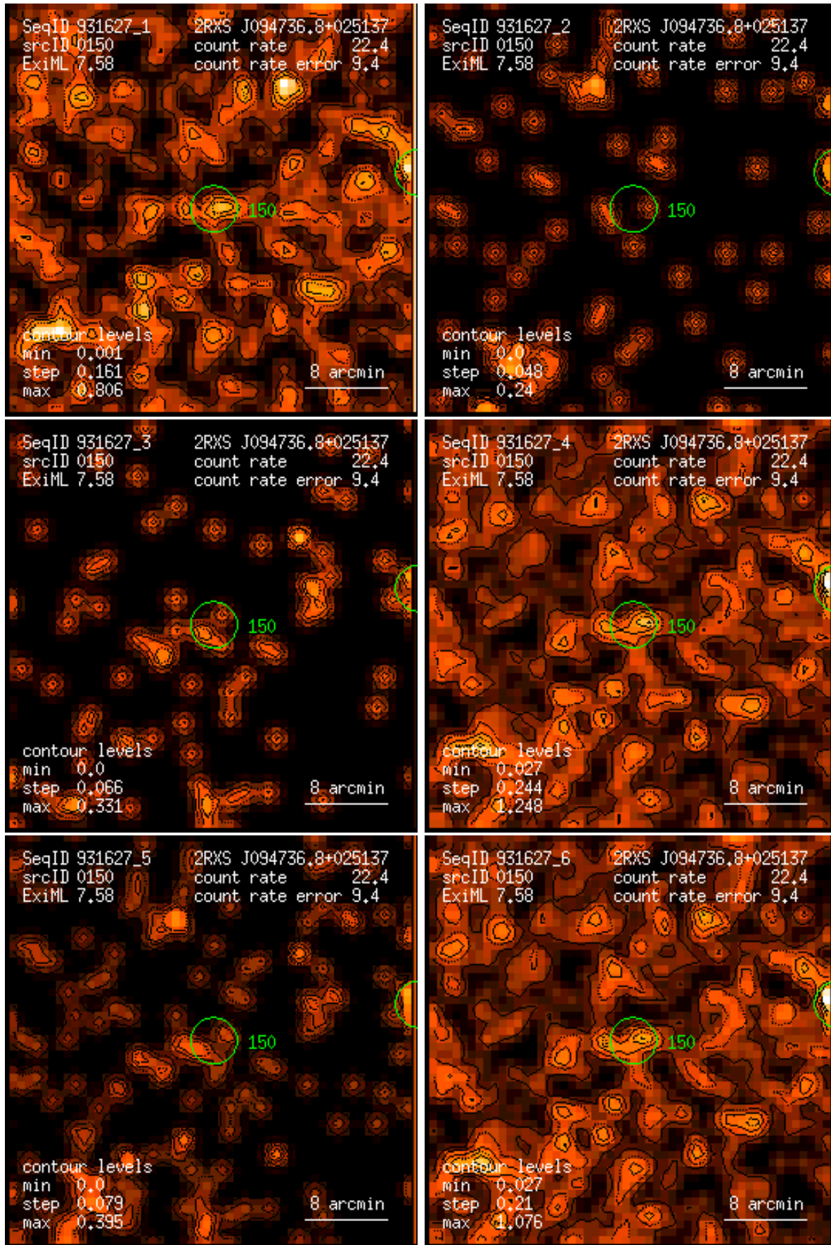
Figure 150: RASS 931627: detection 0150: band rate images, Gaussian filter: (1) PSPC channels 11 – 41, (2) 52 – 90, (3) 91 – 201, (4) 11 – 235, (5) 52 – 201, (6) 11 – 201. Broad band rates in counts/ks. Band rate contour levels in counts/ks/arcmin 2 .
