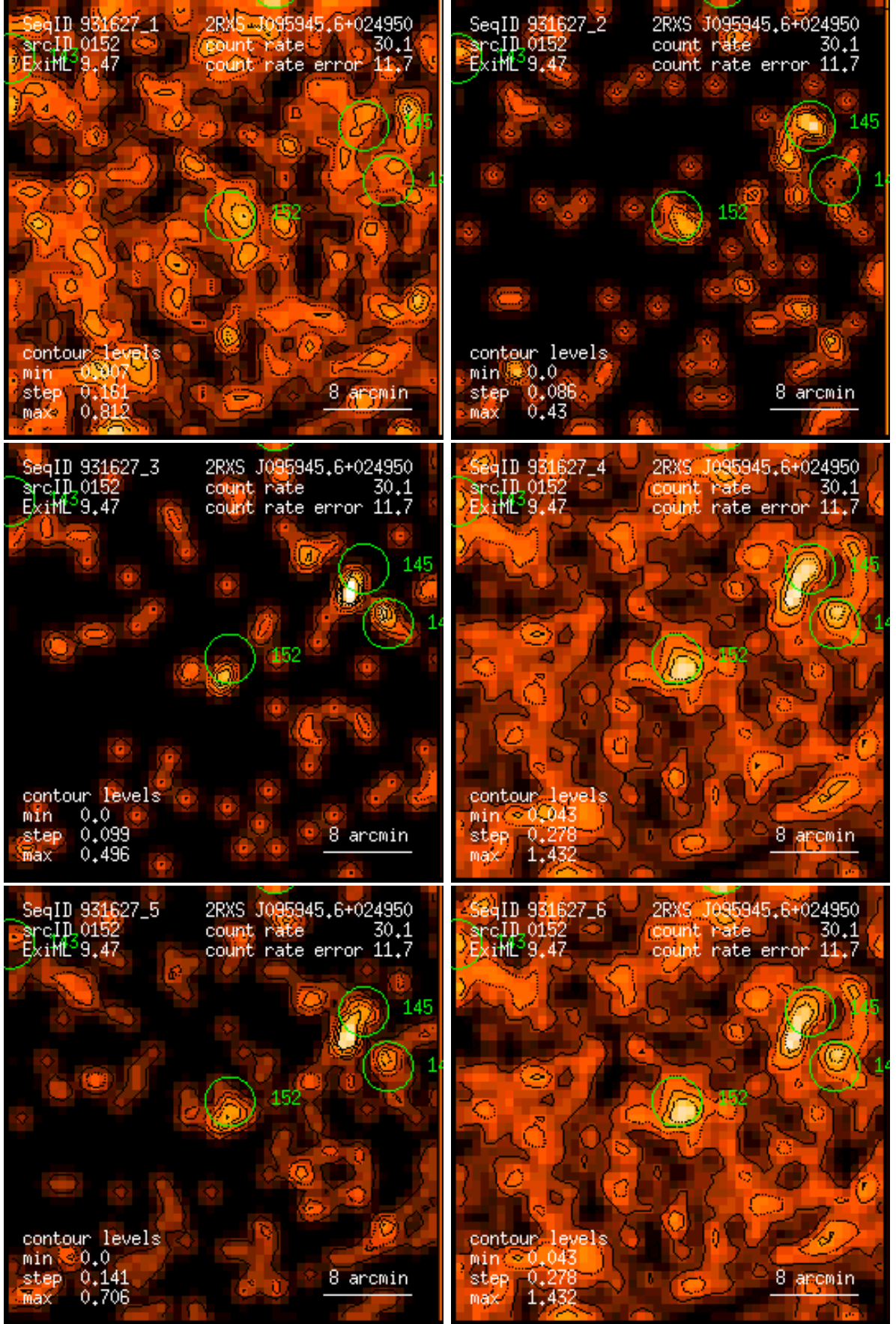
Figure 152: RASS 931627: detection 0152: band rate images, Gaussian filter: (1) PSPC channels 11 – 41, (2) 52 – 90, (3) 91 – 201, (4) 11 – 235, (5) 52 – 201, (6) 11 – 201. Broad band rates in counts/ks. Band rate contour levels in counts/ks/arcmin 2 .
