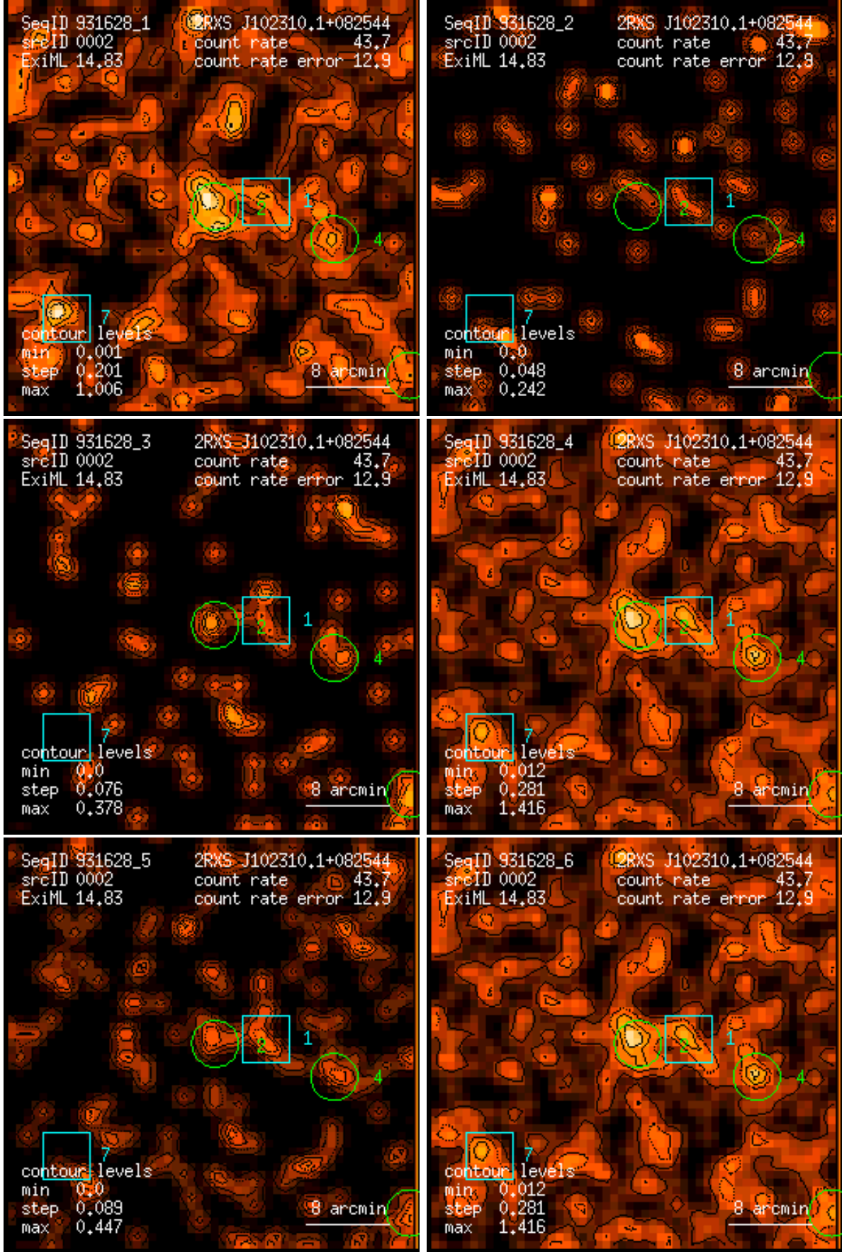
Figure 2: RASS 931628: detection 0002: band rate images, Gaussian filter: (1) PSPC channels 11 – 41, (2) 52 – 90, (3) 91 – 201, (4) 11 – 235, (5) 52 – 201, (6) 11 – 201. Broad band rates in counts/ks. Band rate contour levels in counts/ks/arcmin 2 .
