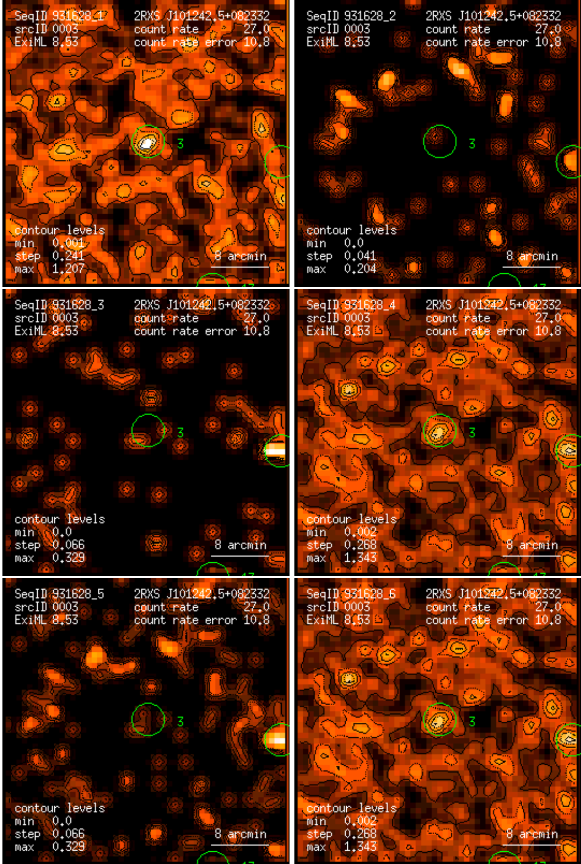
Figure 3: RASS 931628: detection 0003: band rate images, Gaussian filter: (1) PSPC channels 11 – 41, (2) 52 – 90, (3) 91 – 201, (4) 11 – 235, (5) 52 – 201, (6) 11 – 201. Broad band rates in counts/ks. Band rate contour levels in counts/ks/arcmin 2 .
