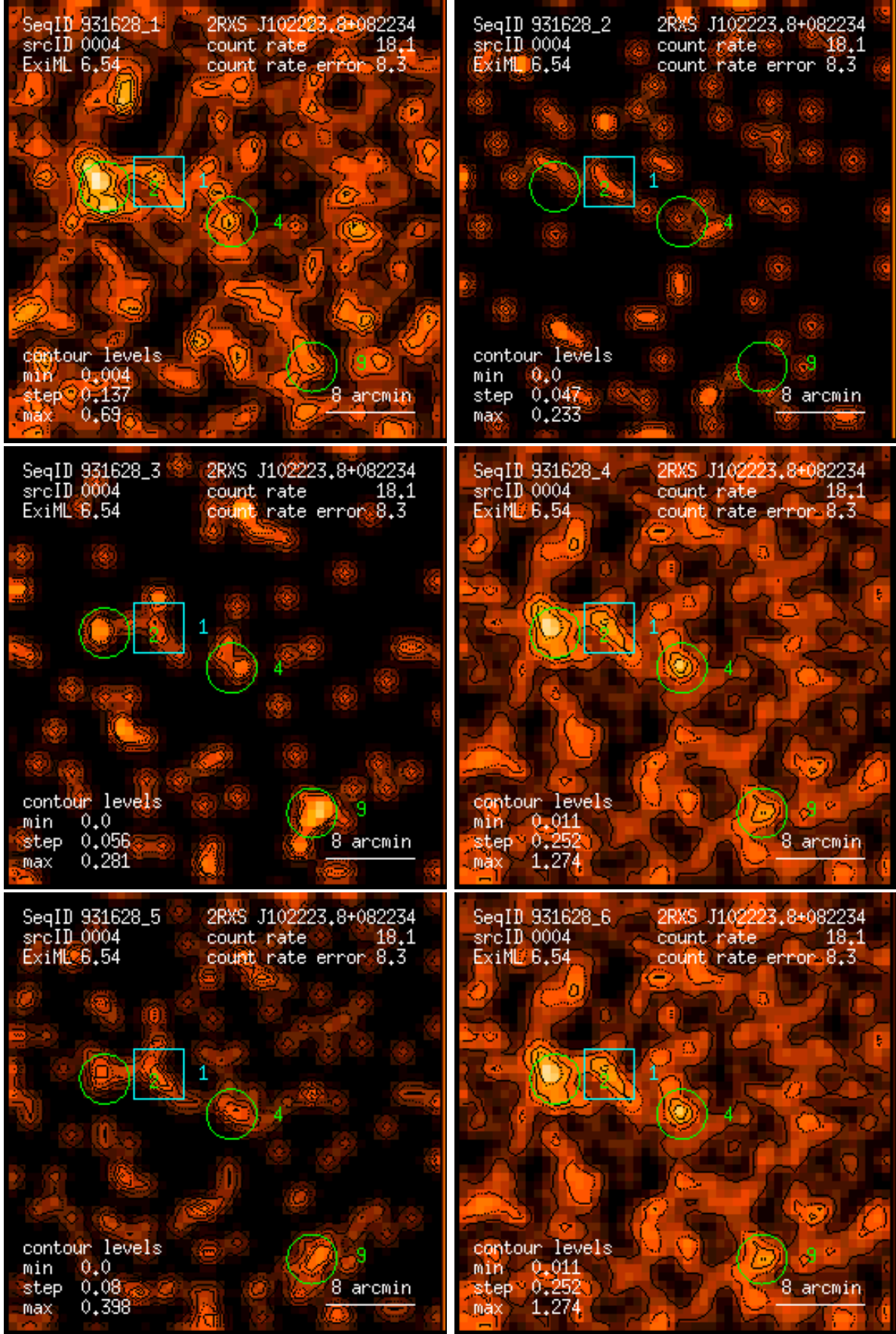
Figure 4: RASS 931628: detection 0004: band rate images, Gaussian filter: (1) PSPC channels 11 – 41, (2) 52 – 90, (3) 91 – 201, (4) 11 – 235, (5) 52 – 201, (6) 11 – 201. Broad band rates in counts/ks. Band rate contour levels in counts/ks/arcmin 2 .
