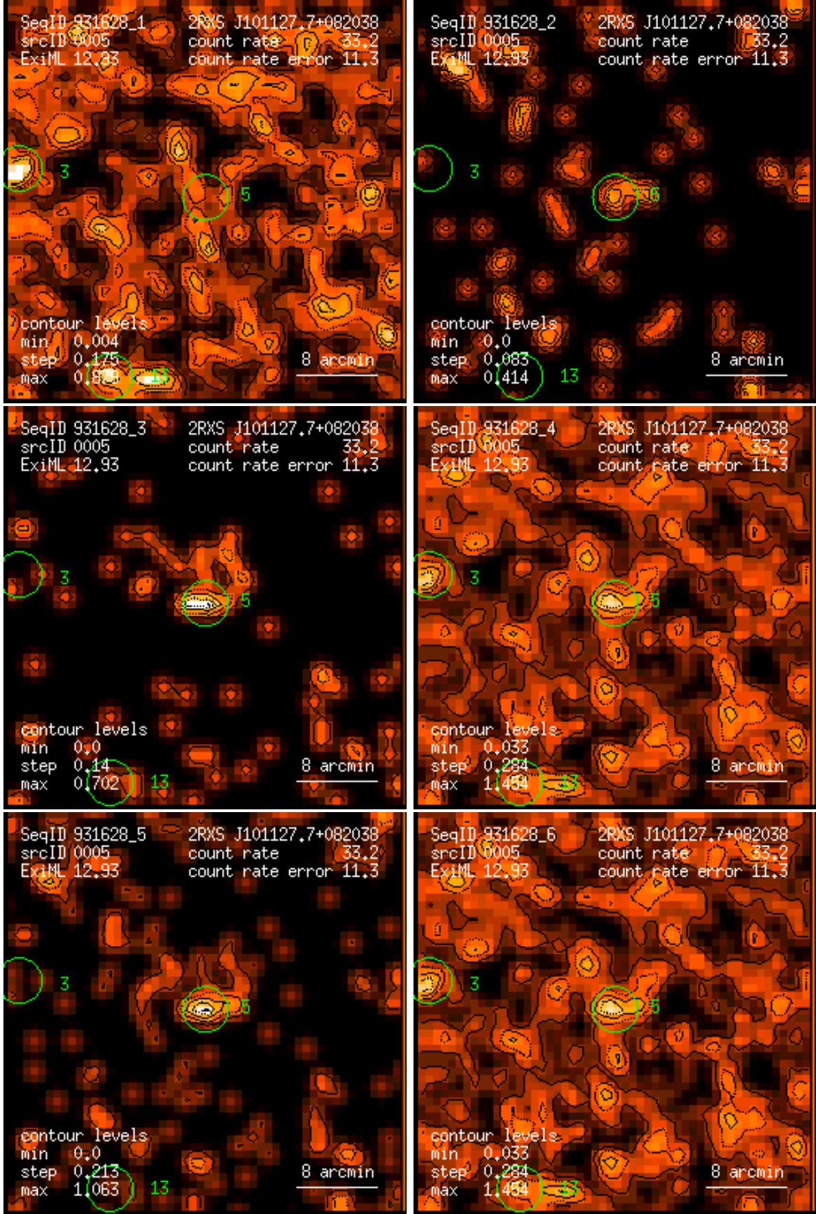
Figure 5: RASS 931628: detection 0005: band rate images, Gaussian filter: (1) PSPC channels 11 – 41, (2) 52 – 90, (3) 91 – 201, (4) 11 – 235, (5) 52 – 201, (6) 11 – 201. Broad band rates in counts/ks. Band rate contour levels in counts/ks/arcmin 2 .
