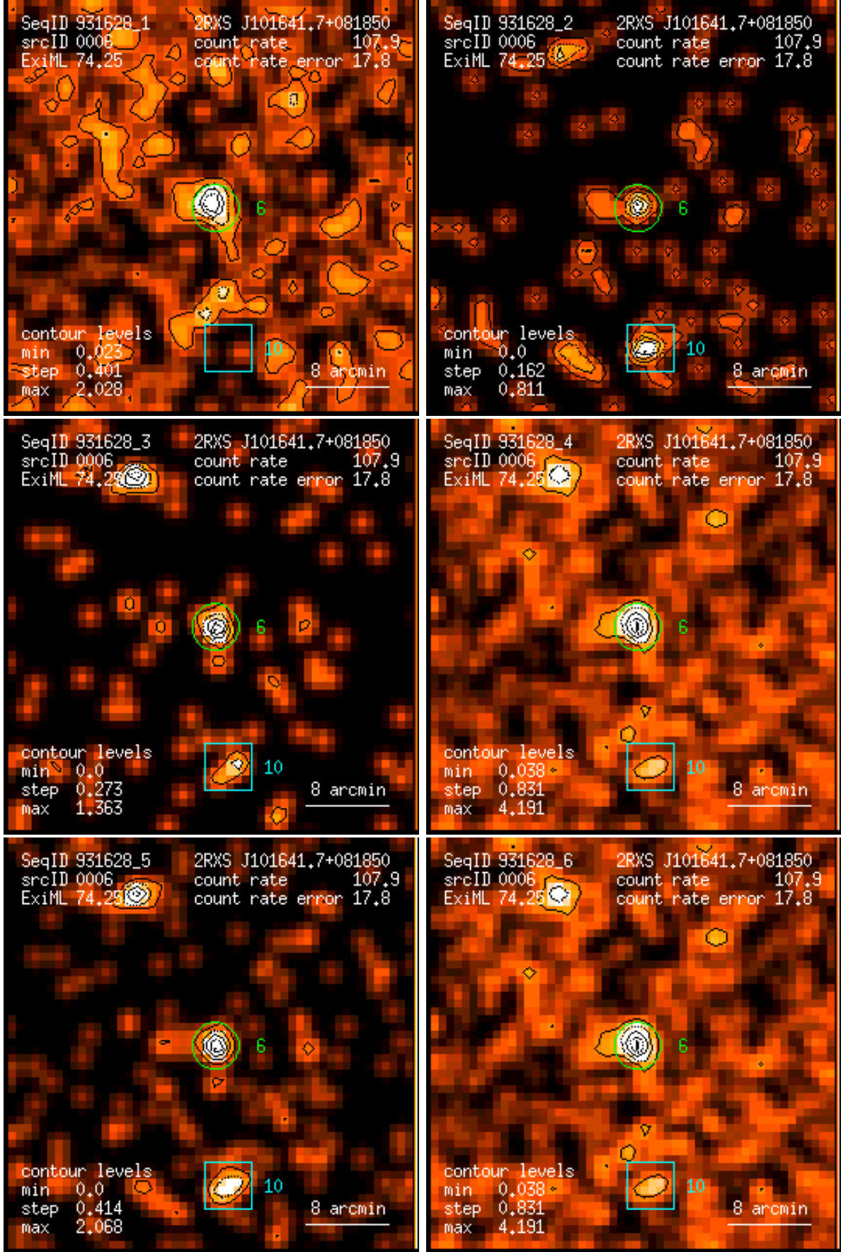
Figure 6: RASS 931628: detection 0006: band rate images, Gaussian filter: (1) PSPC channels 11 – 41, (2) 52 – 90, (3) 91 – 201, (4) 11 – 235, (5) 52 – 201, (6) 11 – 201. Broad band rates in counts/ks. Band rate contour levels in counts/ks/arcmin 2 .
