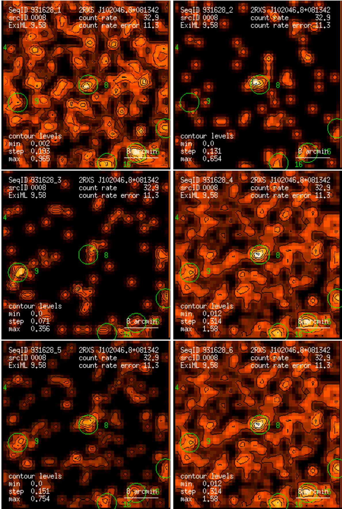
Figure 8: RASS 931628: detection 0008: band rate images, Gaussian filter: (1) PSPC channels 11 – 41, (2) 52 – 90, (3) 91 – 201, (4) 11 – 235, (5) 52 – 201, (6) 11 – 201. Broad band rates in counts/ks. Band rate contour levels in counts/ks/arcmin 2 .
