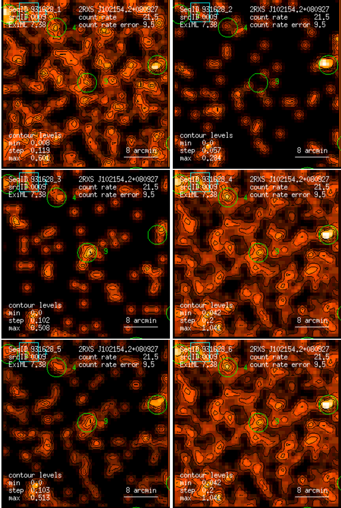
Figure 9: RASS 931628: detection 0009: band rate images, Gaussian filter: (1) PSPC channels 11 – 41, (2) 52 – 90, (3) 91 – 201, (4) 11 – 235, (5) 52 – 201, (6) 11 – 201. Broad band rates in counts/ks. Band rate contour levels in counts/ks/arcmin 2 .
