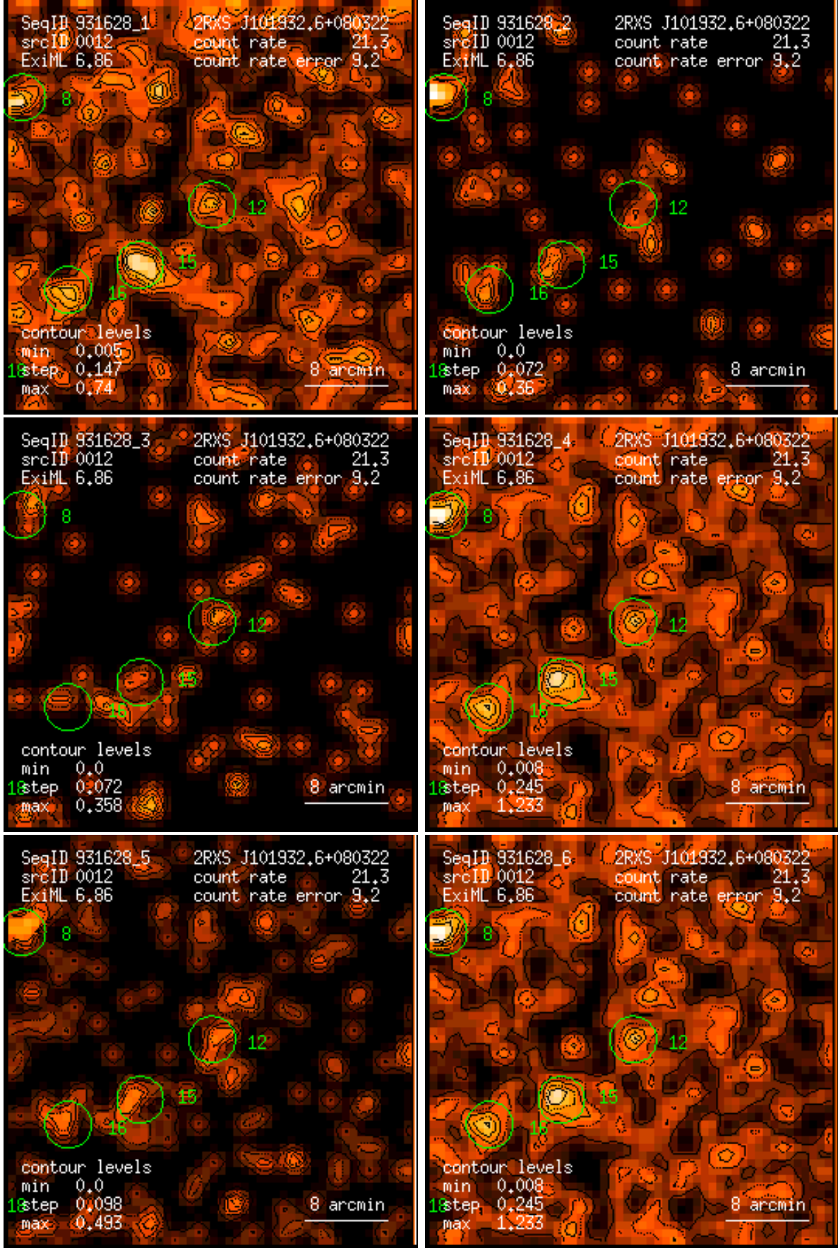
Figure 12: RASS 931628: detection 0012: band rate images, Gaussian filter: (1) PSPC channels 11 – 41, (2) 52 – 90, (3) 91 – 201, (4) 11 – 235, (5) 52 – 201, (6) 11 – 201. Broad band rates in counts/ks. Band rate contour levels in counts/ks/arcmin 2 .
