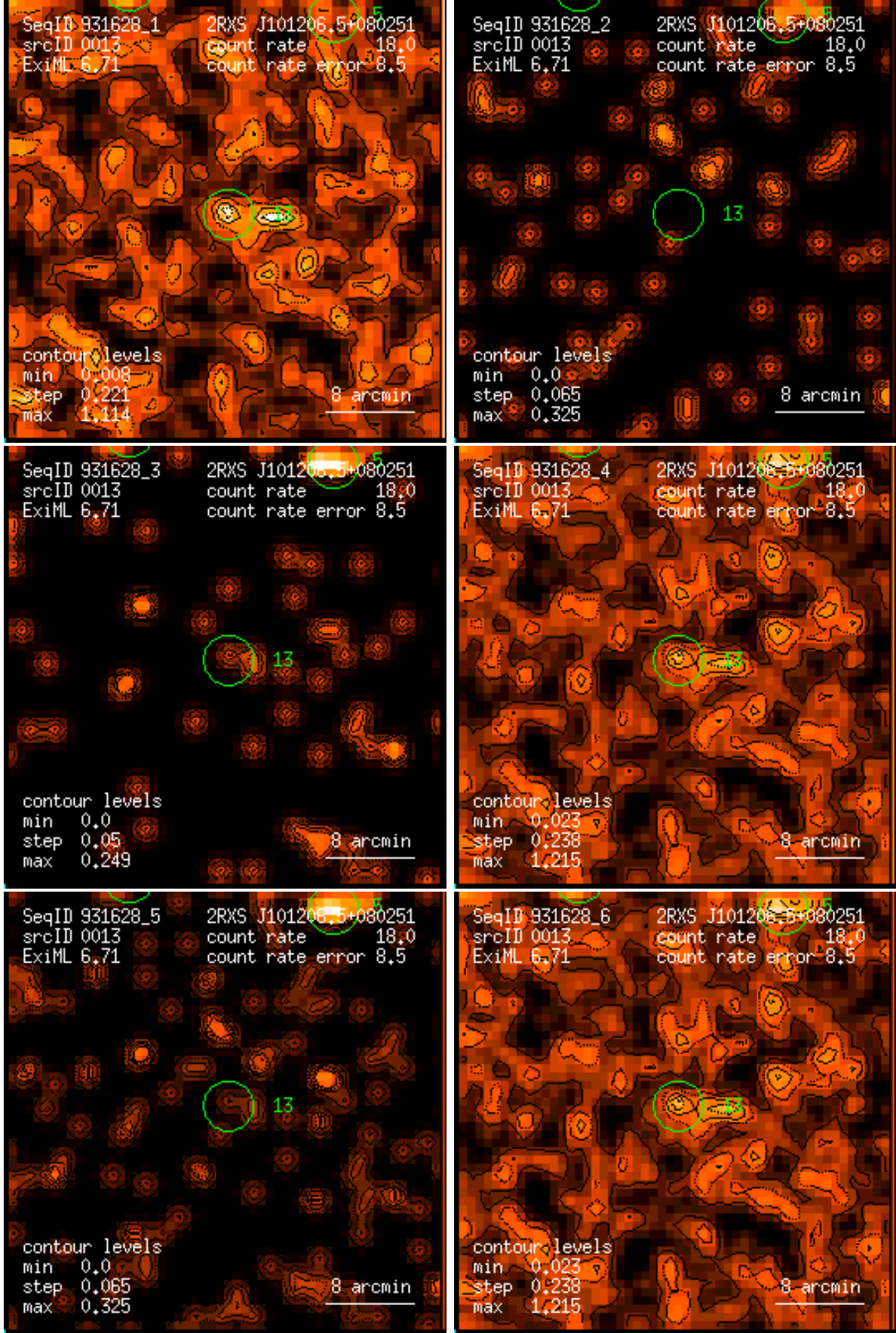
Figure 13: RASS 931628: detection 0013: band rate images, Gaussian filter: (1) PSPC channels 11 – 41, (2) 52 – 90, (3) 91 – 201, (4) 11 – 235, (5) 52 – 201, (6) 11 – 201. Broad band rates in counts/ks. Band rate contour levels in counts/ks/arcmin 2 .
