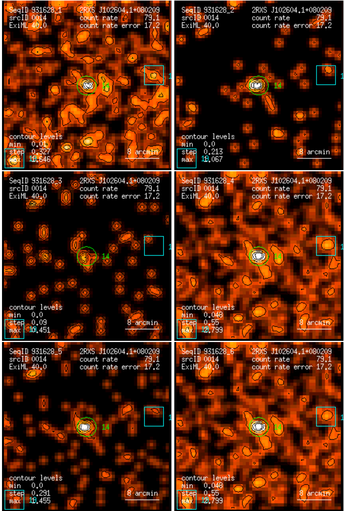
Figure 14: RASS 931628: detection 0014: band rate images, Gaussian filter: (1) PSPC channels 11 – 41, (2) 52 – 90, (3) 91 – 201, (4) 11 – 235, (5) 52 – 201, (6) 11 – 201. Broad band rates in counts/ks. Band rate contour levels in counts/ks/arcmin 2 .
