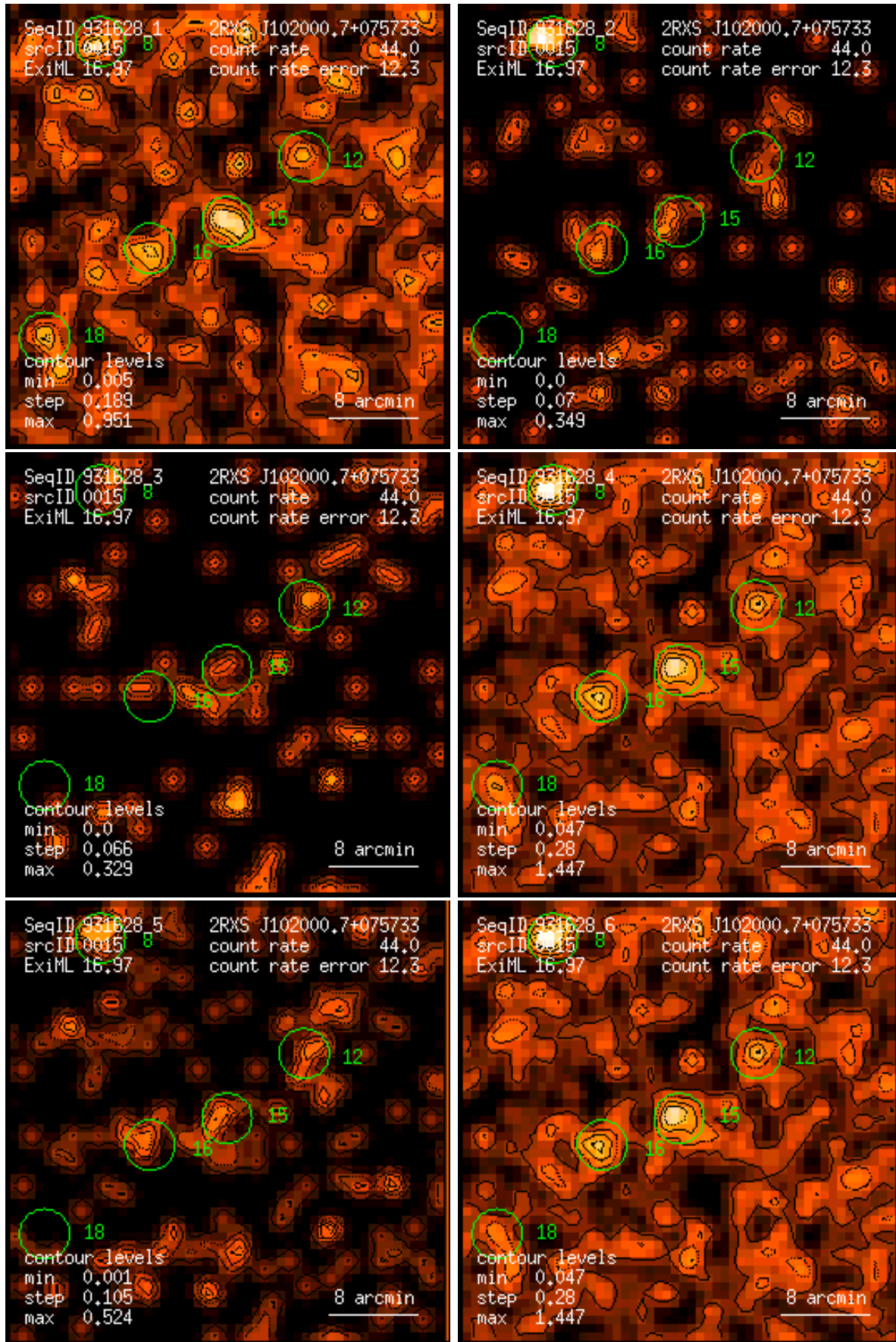
Figure 15: RASS 931628: detection 0015: band rate images, Gaussian filter: (1) PSPC channels 11 – 41, (2) 52 – 90, (3) 91 – 201, (4) 11 – 235, (5) 52 – 201, (6) 11 – 201. Broad band rates in counts/ks. Band rate contour levels in counts/ks/arcmin 2 .
