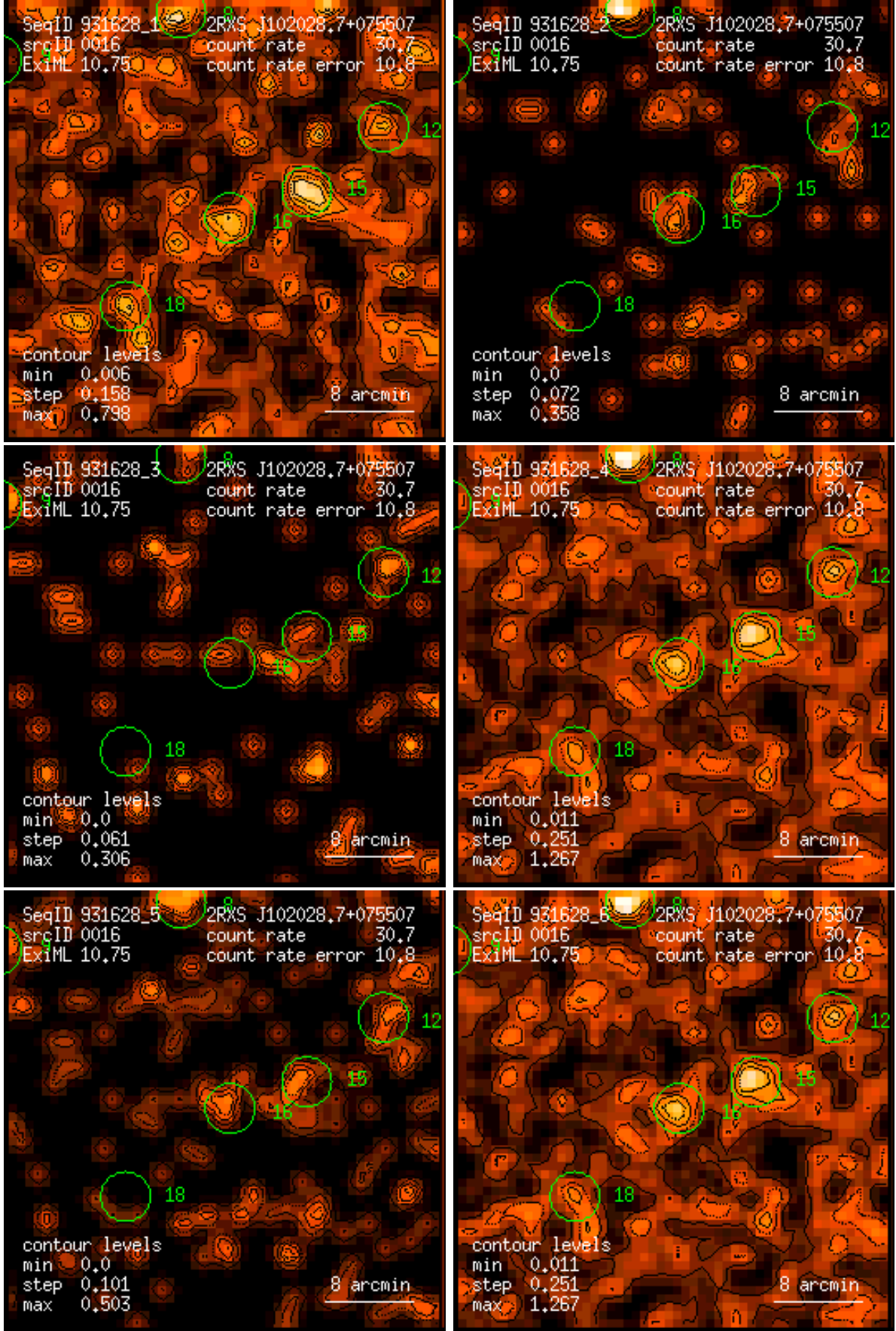
Figure 16: RASS 931628: detection 0016: band rate images, Gaussian filter: (1) PSPC channels 11 – 41, (2) 52 – 90, (3) 91 – 201, (4) 11 – 235, (5) 52 – 201, (6) 11 – 201. Broad band rates in counts/ks. Band rate contour levels in counts/ks/arcmin 2 .
