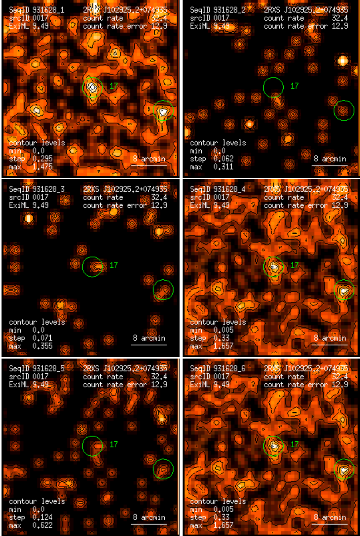
Figure 17: RASS 931628: detection 0017: band rate images, Gaussian filter: (1) PSPC channels 11 – 41, (2) 52 – 90, (3) 91 – 201, (4) 11 – 235, (5) 52 – 201, (6) 11 – 201. Broad band rates in counts/ks. Band rate contour levels in counts/ks/arcmin 2 .
