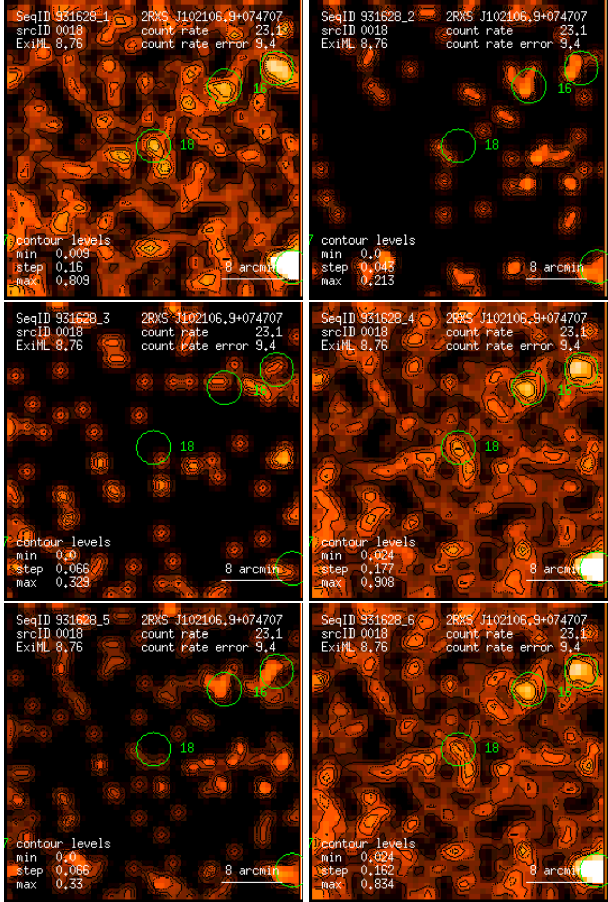
Figure 18: RASS 931628: detection 0018: band rate images, Gaussian filter: (1) PSPC channels 11 – 41, (2) 52 – 90, (3) 91 – 201, (4) 11 – 235, (5) 52 – 201, (6) 11 – 201. Broad band rates in counts/ks. Band rate contour levels in counts/ks/arcmin 2 .
