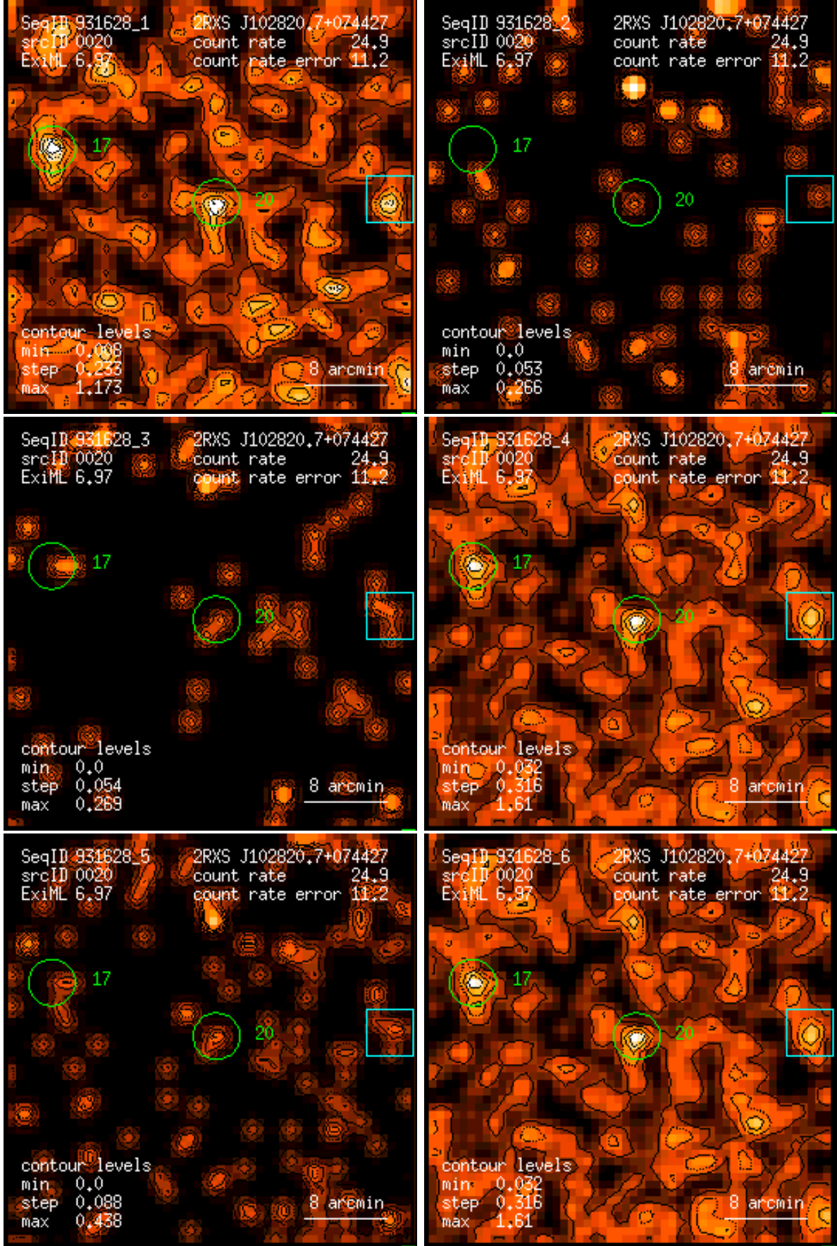
Figure 20: RASS 931628: detection 0020: band rate images, Gaussian filter: (1) PSPC channels 11 – 41, (2) 52 – 90, (3) 91 – 201, (4) 11 – 235, (5) 52 – 201, (6) 11 – 201. Broad band rates in counts/ks. Band rate contour levels in counts/ks/arcmin 2 .
