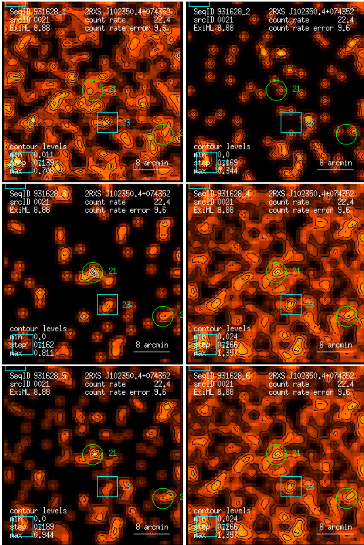
Figure 21: RASS 931628: detection 0021: band rate images, Gaussian filter: (1) PSPC channels 11 – 41, (2) 52 – 90, (3) 91 – 201, (4) 11 – 235, (5) 52 – 201, (6) 11 – 201. Broad band rates in counts/ks. Band rate contour levels in counts/ks/arcmin 2 .
