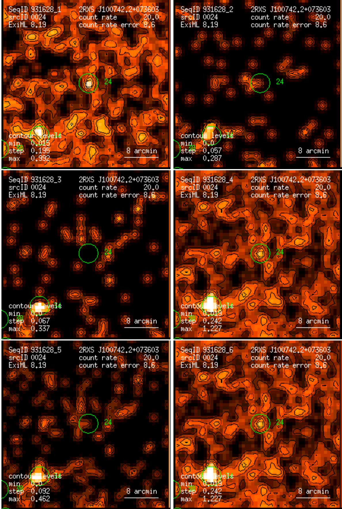
Figure 24: RASS 931628: detection 0024: band rate images, Gaussian filter: (1) PSPC channels 11 – 41, (2) 52 – 90, (3) 91 – 201, (4) 11 – 235, (5) 52 – 201, (6) 11 – 201. Broad band rates in counts/ks. Band rate contour levels in counts/ks/arcmin 2 .
