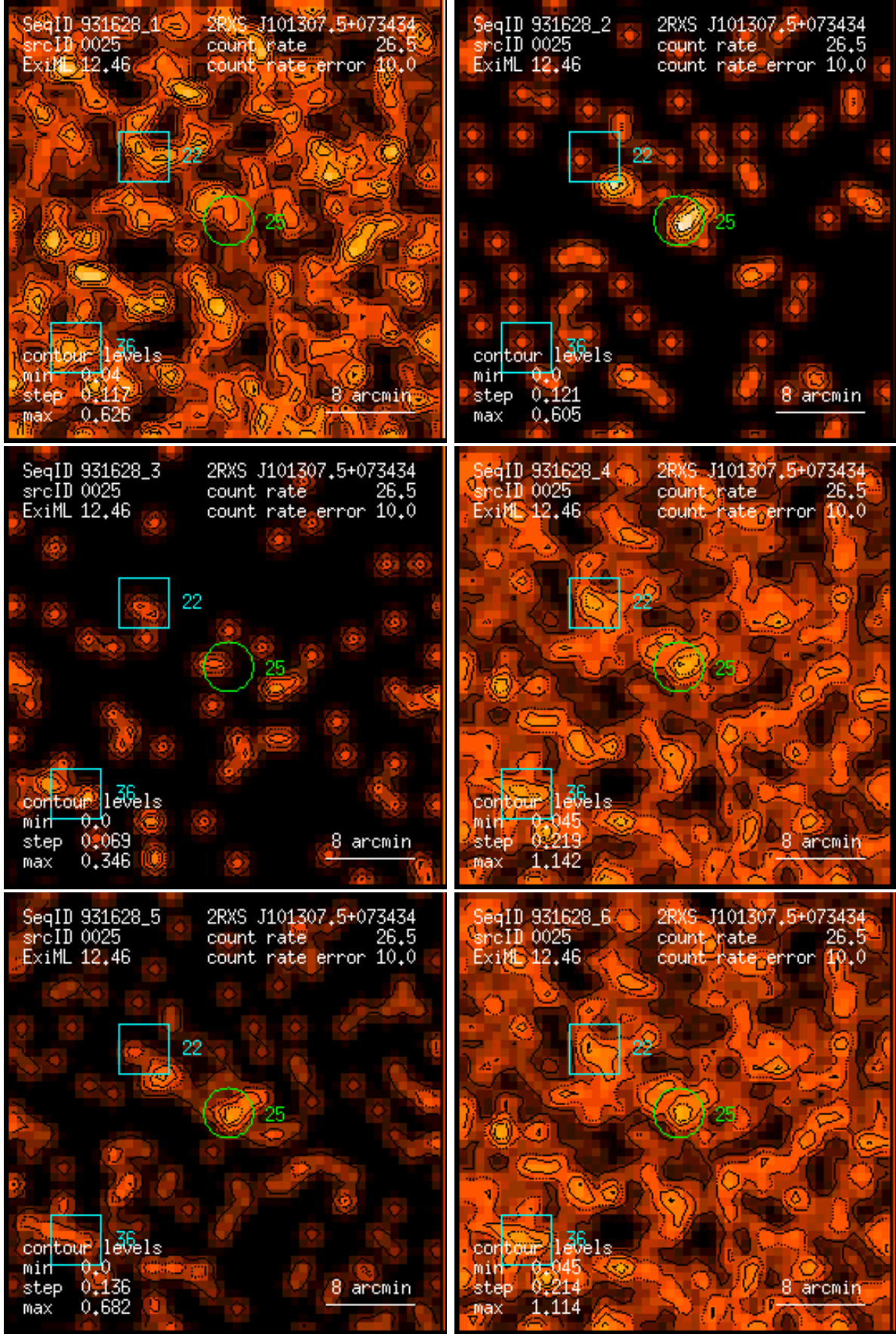
Figure 25: RASS 931628: detection 0025: band rate images, Gaussian filter: (1) PSPC channels 11 – 41, (2) 52 – 90, (3) 91 – 201, (4) 11 – 235, (5) 52 – 201, (6) 11 – 201. Broad band rates in counts/ks. Band rate contour levels in counts/ks/arcmin 2 .
