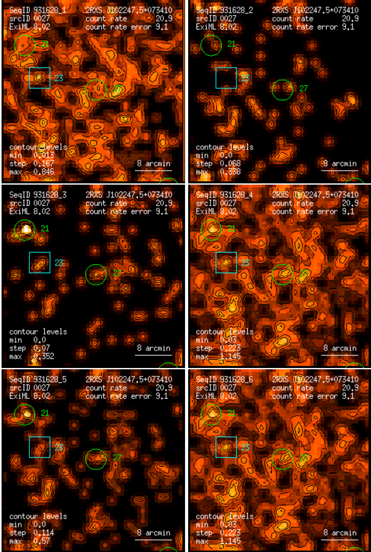
Figure 27: RASS 931628: detection 0027: band rate images, Gaussian filter: (1) PSPC channels 11 – 41, (2) 52 – 90, (3) 91 – 201, (4) 11 – 235, (5) 52 – 201, (6) 11 – 201. Broad band rates in counts/ks. Band rate contour levels in counts/ks/arcmin 2 .
