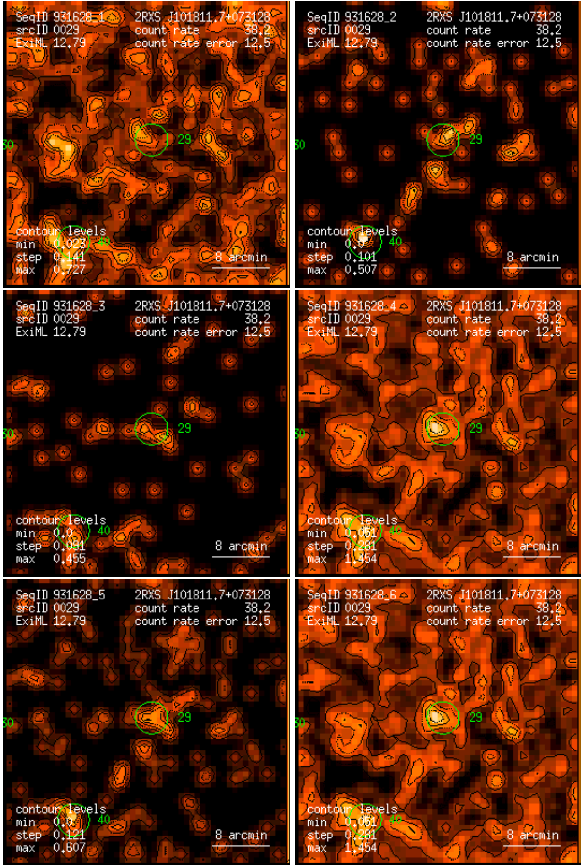
Figure 29: RASS 931628: detection 0029: band rate images, Gaussian filter: (1) PSPC channels 11 – 41, (2) 52 – 90, (3) 91 – 201, (4) 11 – 235, (5) 52 – 201, (6) 11 – 201. Broad band rates in counts/ks. Band rate contour levels in counts/ks/arcmin 2 .
