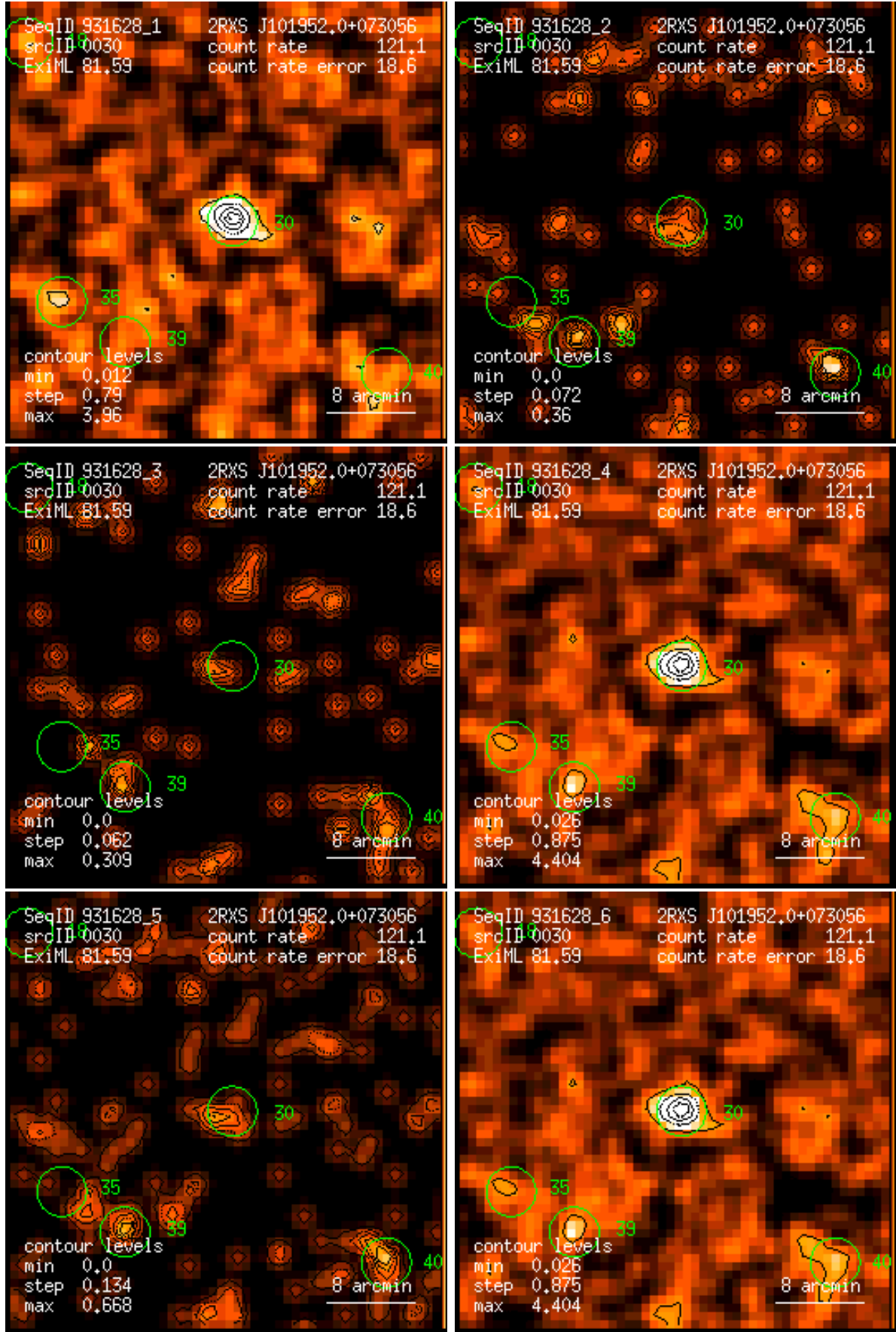
Figure 30: RASS 931628: detection 0030: band rate images, Gaussian filter: (1) PSPC channels 11 – 41, (2) 52 – 90, (3) 91 – 201, (4) 11 – 235, (5) 52 – 201, (6) 11 – 201. Broad band rates in counts/ks. Band rate contour levels in counts/ks/arcmin 2 .
