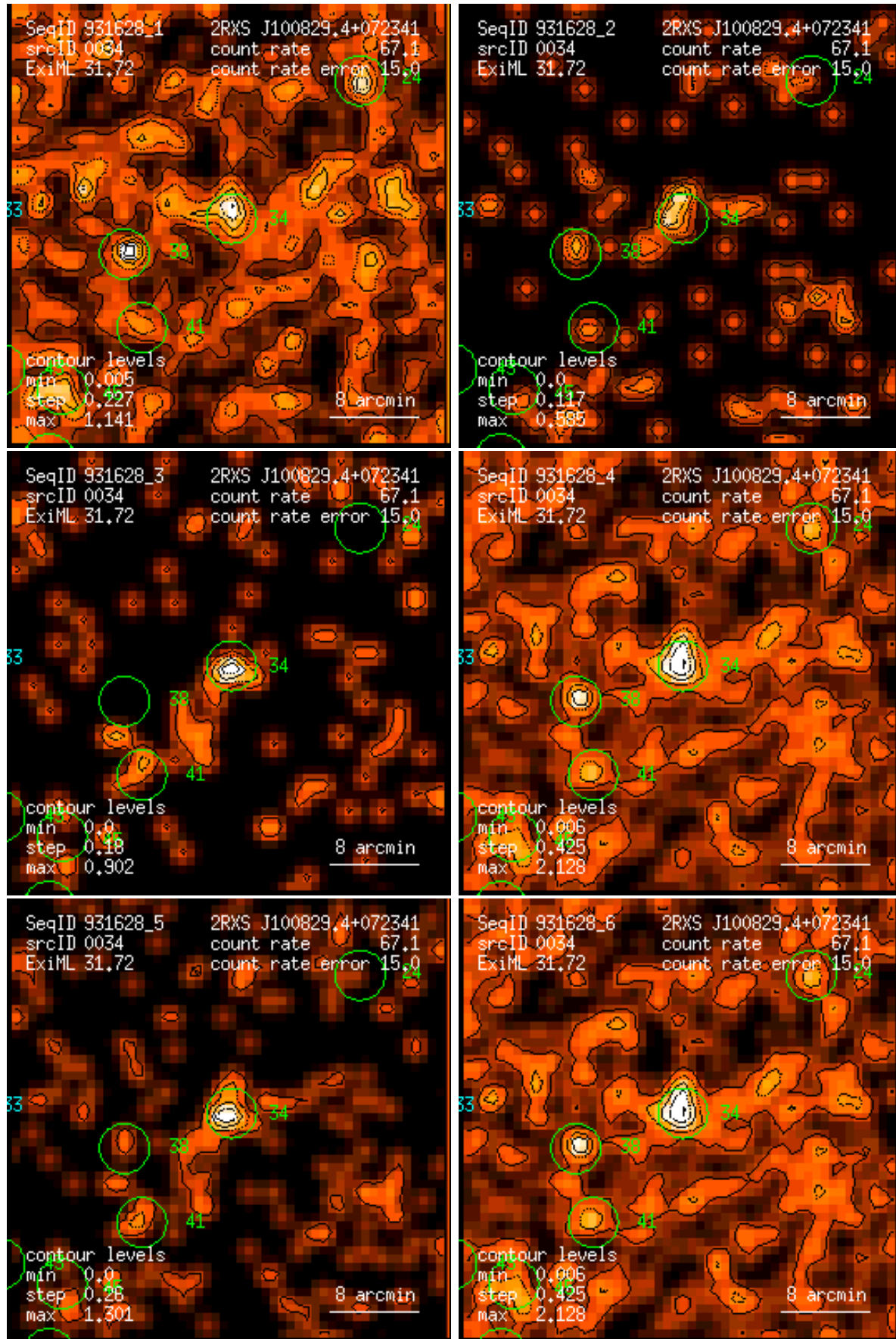
Figure 34: RASS 931628: detection 0034: band rate images, Gaussian filter: (1) PSPC channels 11 – 41, (2) 52 – 90, (3) 91 – 201, (4) 11 – 235, (5) 52 – 201, (6) 11 – 201. Broad band rates in counts/ks. Band rate contour levels in counts/ks/arcmin 2 .
