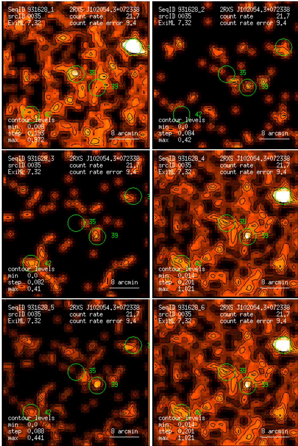
Figure 35: RASS 931628: detection 0035: band rate images, Gaussian filter: (1) PSPC channels 11 – 41, (2) 52 – 90, (3) 91 – 201, (4) 11 – 235, (5) 52 – 201, (6) 11 – 201. Broad band rates in counts/ks. Band rate contour levels in counts/ks/arcmin 2 .
