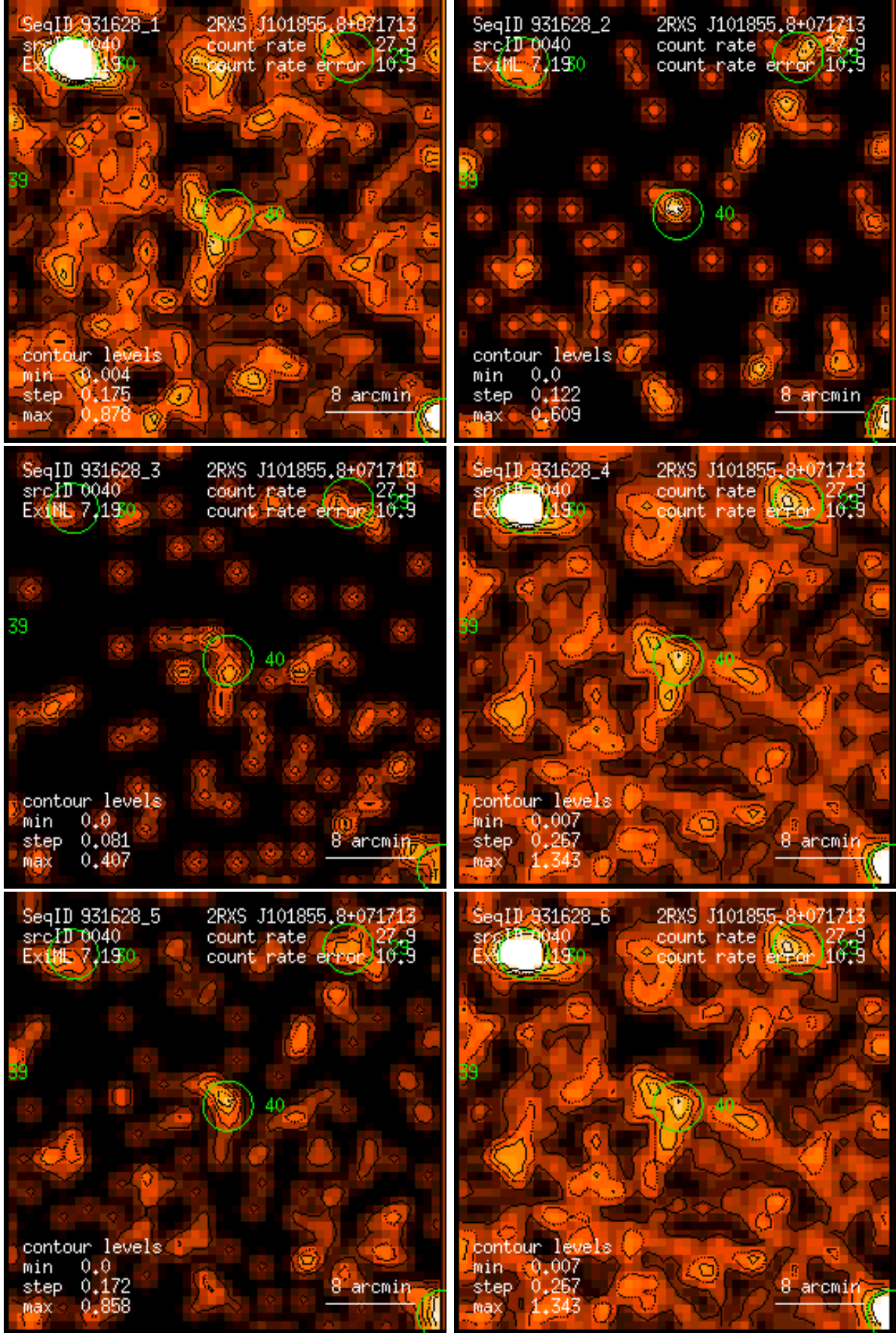
Figure 40: RASS 931628: detection 0040: band rate images, Gaussian filter: (1) PSPC channels 11 – 41, (2) 52 – 90, (3) 91 – 201, (4) 11 – 235, (5) 52 – 201, (6) 11 – 201. Broad band rates in counts/ks. Band rate contour levels in counts/ks/arcmin 2 .
