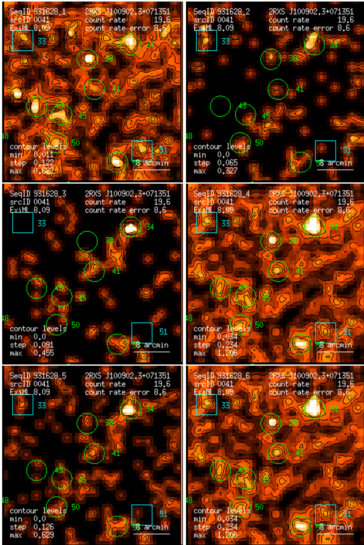
Figure 41: RASS 931628: detection 0041: band rate images, Gaussian filter: (1) PSPC channels 11 – 41, (2) 52 – 90, (3) 91 – 201, (4) 11 – 235, (5) 52 – 201, (6) 11 – 201. Broad band rates in counts/ks. Band rate contour levels in counts/ks/arcmin 2 .
