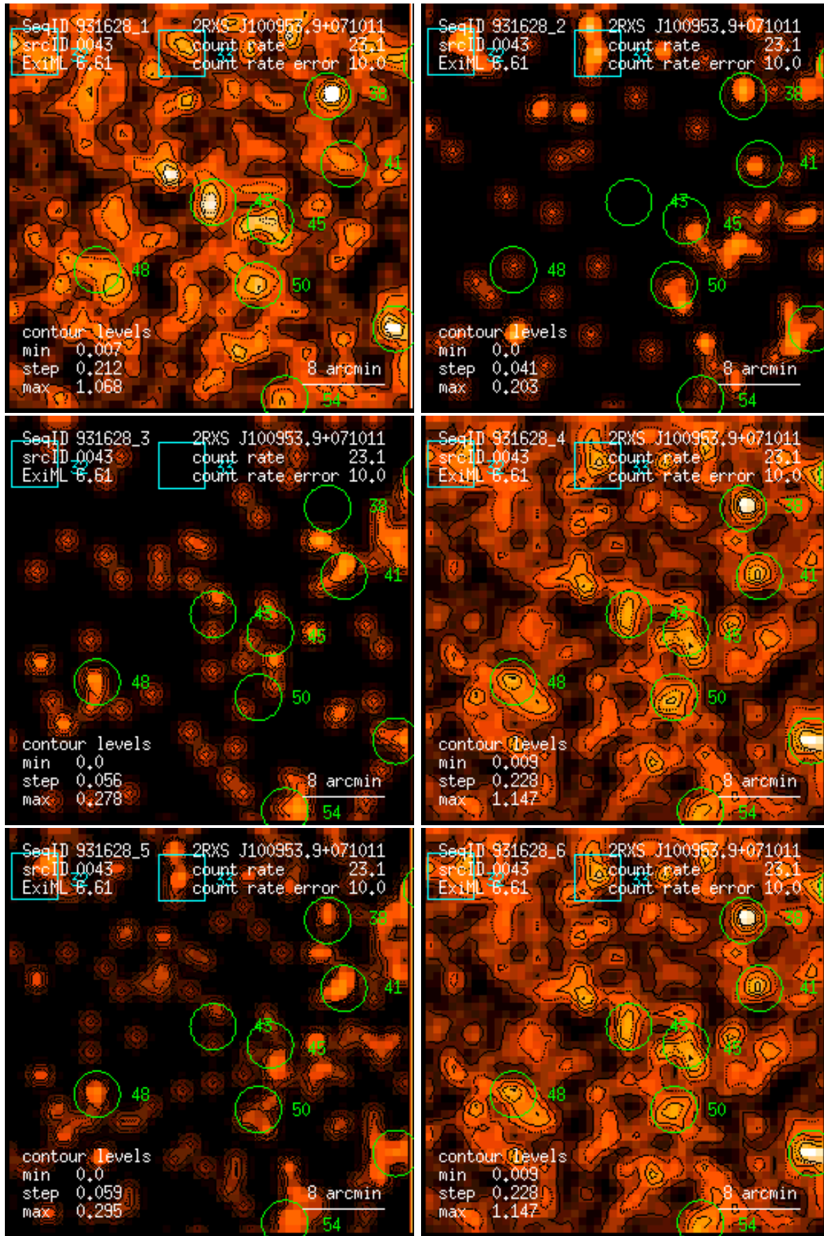
Figure 43: RASS 931628: detection 0043: band rate images, Gaussian filter: (1) PSPC channels 11 – 41, (2) 52 – 90, (3) 91 – 201, (4) 11 – 235, (5) 52 – 201, (6) 11 – 201. Broad band rates in counts/ks. Band rate contour levels in counts/ks/arcmin 2 .
