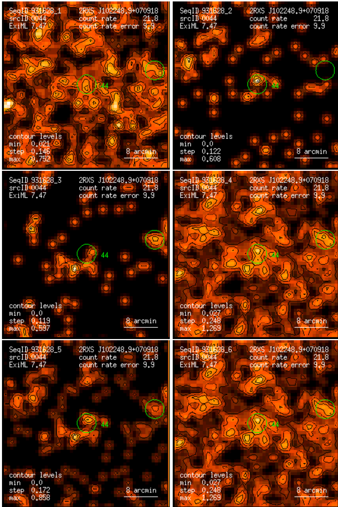
Figure 44: RASS 931628: detection 0044: band rate images, Gaussian filter: (1) PSPC channels 11 – 41, (2) 52 – 90, (3) 91 – 201, (4) 11 – 235, (5) 52 – 201, (6) 11 – 201. Broad band rates in counts/ks. Band rate contour levels in counts/ks/arcmin 2 .
