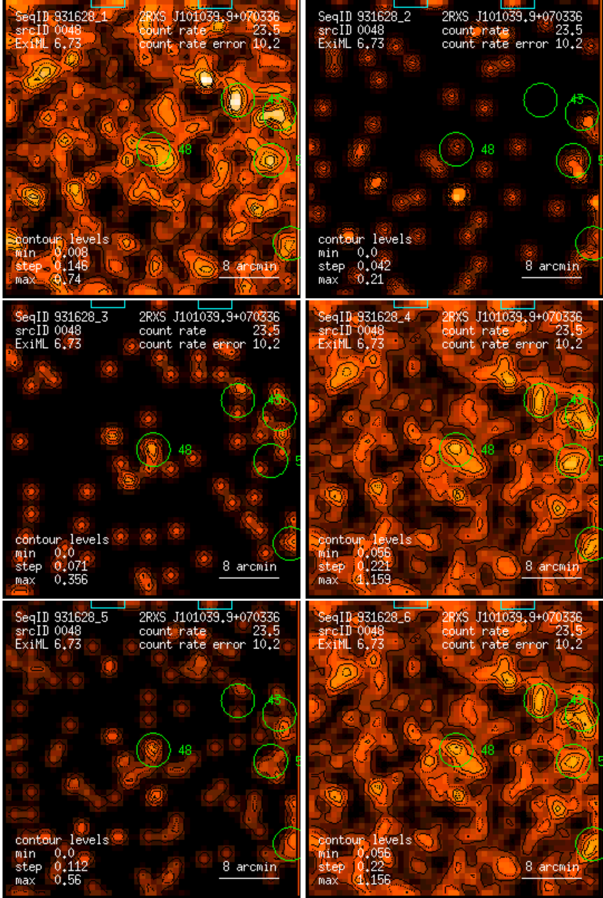
Figure 48: RASS 931628: detection 0048: band rate images, Gaussian filter: (1) PSPC channels 11 – 41, (2) 52 – 90, (3) 91 – 201, (4) 11 – 235, (5) 52 – 201, (6) 11 – 201. Broad band rates in counts/ks. Band rate contour levels in counts/ks/arcmin 2 .
