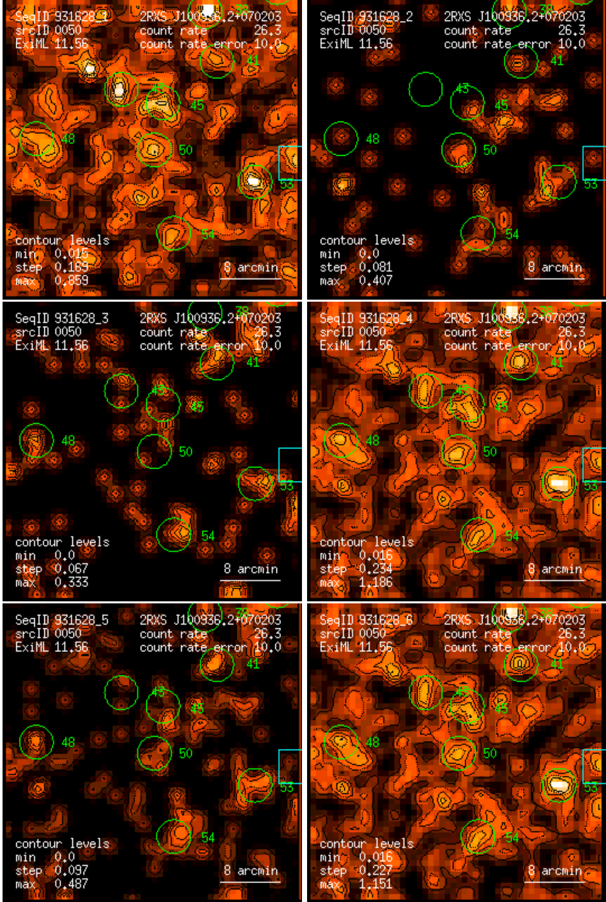
Figure 50: RASS 931628: detection 0050: band rate images, Gaussian filter: (1) PSPC channels 11 – 41, (2) 52 – 90, (3) 91 – 201, (4) 11 – 235, (5) 52 – 201, (6) 11 – 201. Broad band rates in counts/ks. Band rate contour levels in counts/ks/arcmin 2 .
