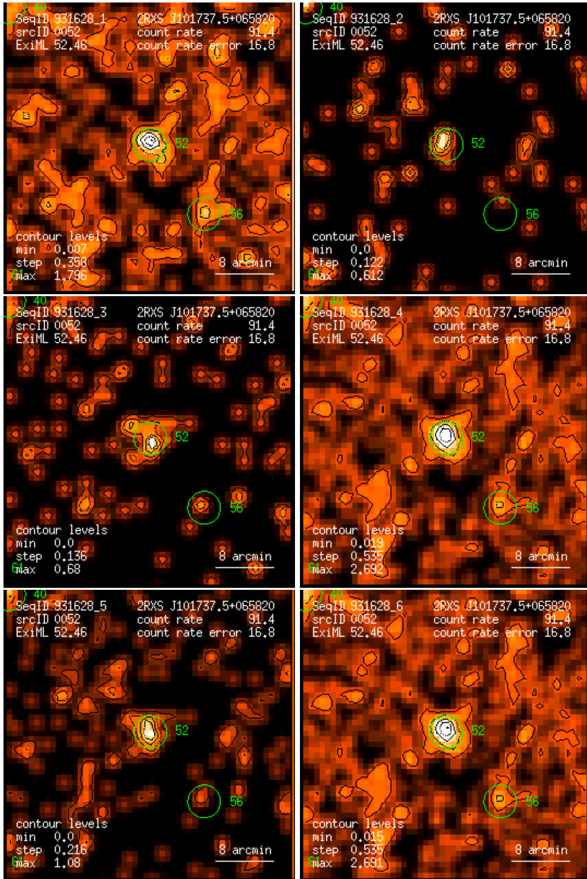
Figure 52: RASS 931628: detection 0052: band rate images, Gaussian filter: (1) PSPC channels 11 – 41, (2) 52 – 90, (3) 91 – 201, (4) 11 – 235, (5) 52 – 201, (6) 11 – 201. Broad band rates in counts/ks. Band rate contour levels in counts/ks/arcmin 2 .
