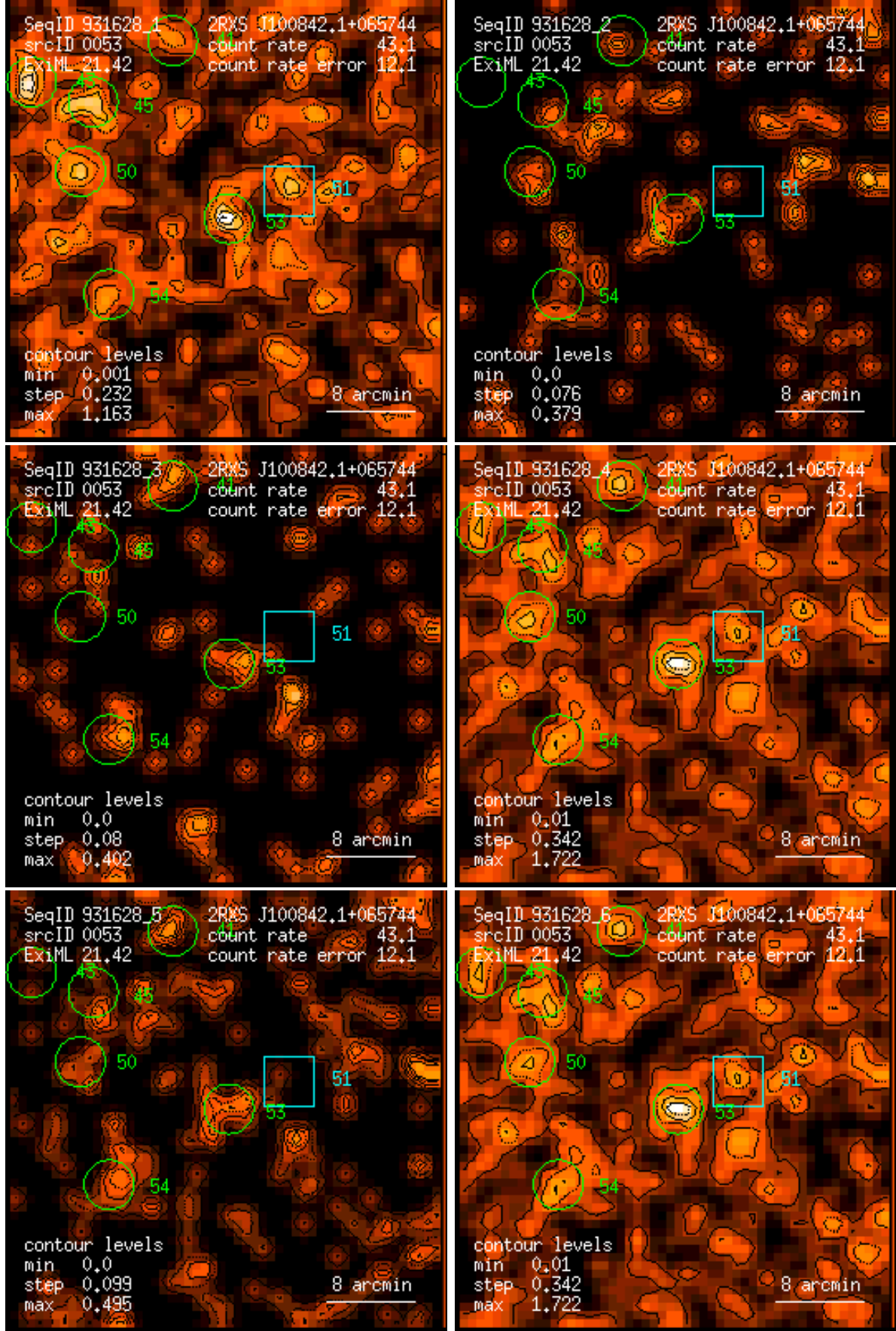
Figure 53: RASS 931628: detection 0053: band rate images, Gaussian filter: (1) PSPC channels 11 – 41, (2) 52 – 90, (3) 91 – 201, (4) 11 – 235, (5) 52 – 201, (6) 11 – 201. Broad band rates in counts/ks. Band rate contour levels in counts/ks/arcmin 2 .
