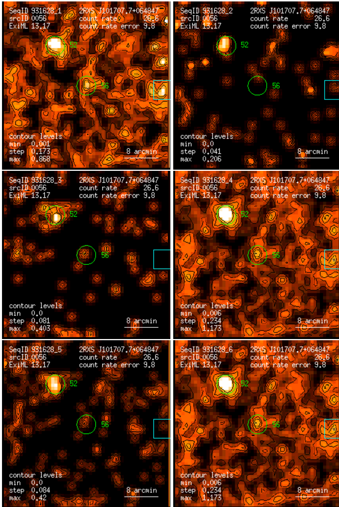
Figure 56: RASS 931628: detection 0056: band rate images, Gaussian filter: (1) PSPC channels 11 – 41, (2) 52 – 90, (3) 91 – 201, (4) 11 – 235, (5) 52 – 201, (6) 11 – 201. Broad band rates in counts/ks. Band rate contour levels in counts/ks/arcmin 2 .
