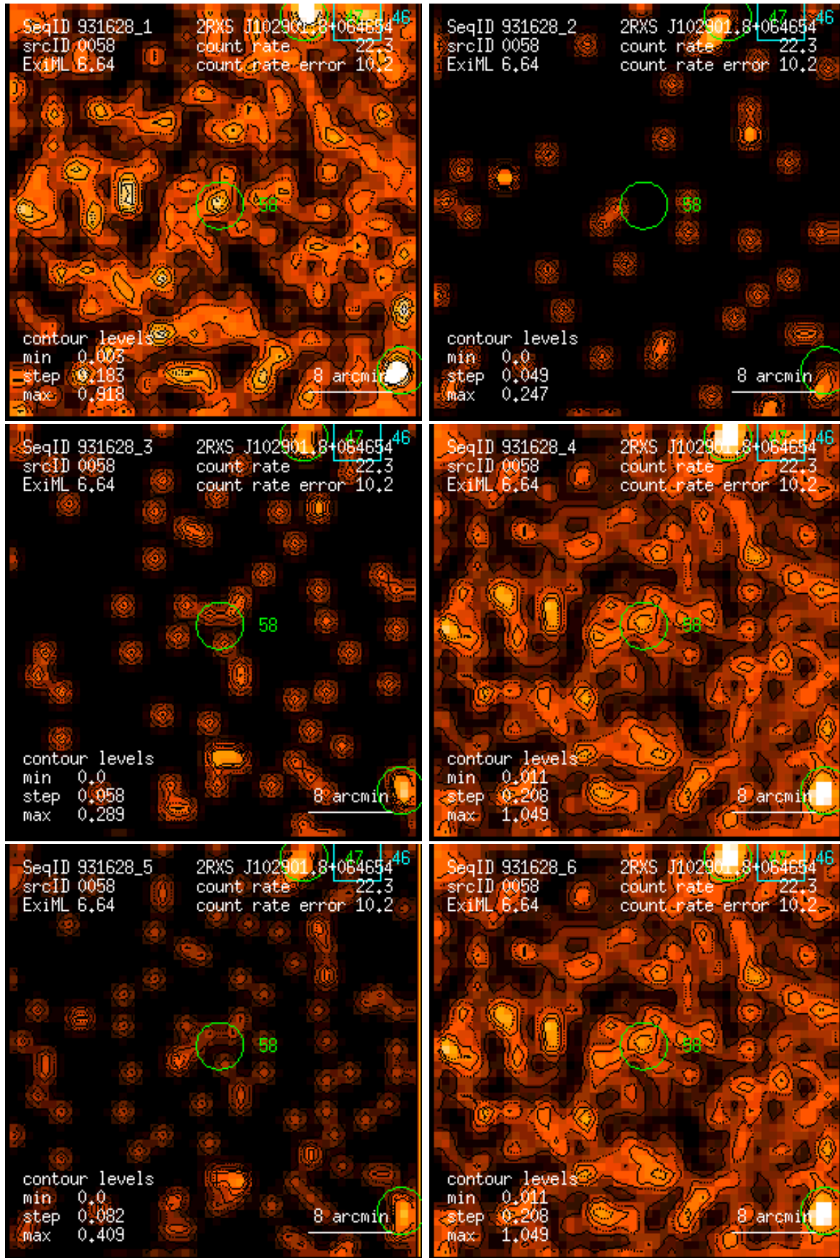
Figure 58: RASS 931628: detection 0058: band rate images, Gaussian filter: (1) PSPC channels 11 – 41, (2) 52 – 90, (3) 91 – 201, (4) 11 – 235, (5) 52 – 201, (6) 11 – 201. Broad band rates in counts/ks. Band rate contour levels in counts/ks/arcmin 2 .
